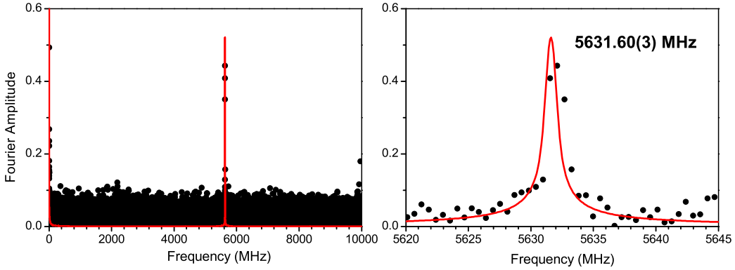
Figure 4: FFT (time window 1.75 \mu\text{s} ) of the hyperfine oscillation signal of muonium in a synthetic quartz crystal in a longitudinal applied field of 0.12 \text{ T} , measured with a dedicated high-time resolution ( \sigma \sim 45 \text{ ps} ) \mu\text{SR} -setup. The red line (detailed view on the right hand side) shows the FFT of the result of a fit of the first 1.75 \mu\text{s} in the time domain, the calculated polarization for this precession is P_{24} = 0.32 .
