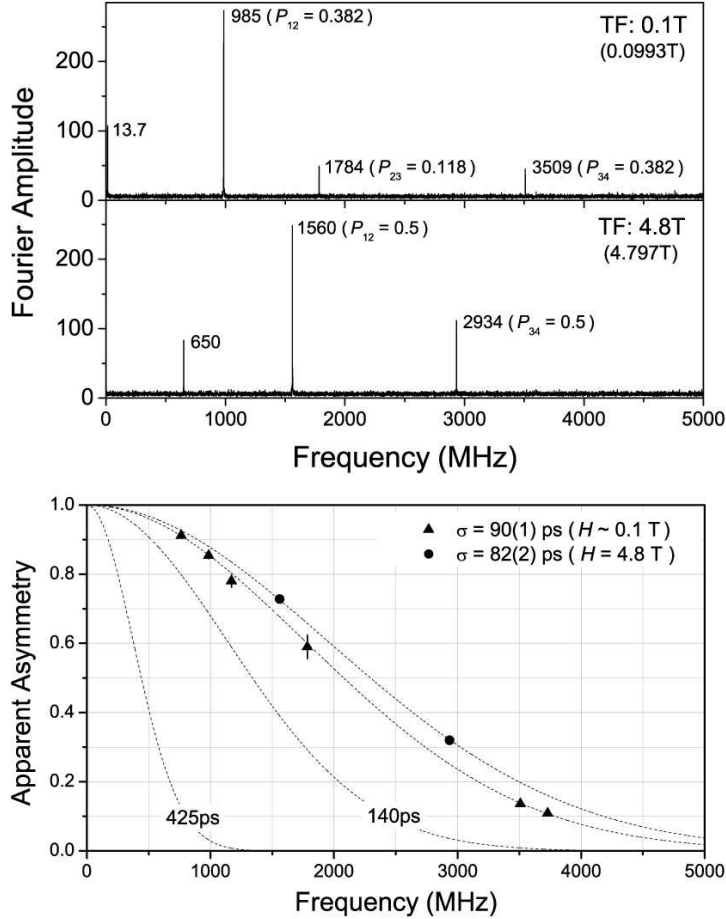
Figure 3: (Top) Fourier spectra in quartz in transverse fields of 0.1 T and 4.8 T. The isotropic part of the hyperfine coupling constant in this crystal at 290 K is 4495.6 MHz. For each muonium signal the calculated polarization P_{ij} is indicated. (Bottom) Reduction of the apparent muonium asymmetry A_{\text{Mu}}(\nu)/A_{\text{Mu}}(0) with increasing the signal frequency measured on a synthetic quartz crystal in transverse magnetic fields of 0.07, 0.1, and 4.8 T. The dashed lines represent the dependence (1) for different values of the time resolution \sigma . For comparison, a characteristic time resolution of a “standard” \mu\text{SR} instrument is \sim 425 ps, and 140 ps is the required time resolution (upper limit) for the 9.5 T instrument at PSI.
