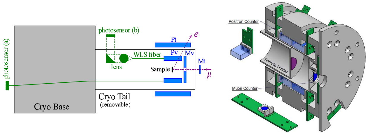
Figure 1: (Left) The sample environment and the detector layout of the High-Field \mu SR instrument. (Right) Prototype of the Timing detector module: design view. Plastic scintillators of type EJ-232 from Eljen are used. Their dimensions: \varnothing 7 \times 0.3 mm (muon counter), 12 \times 12 \times 5 mm (positron counter). Each scintillator is readout by a pair of G-APDs of type MPPC S10362-33-050C from Hamamatsu Photonics.
