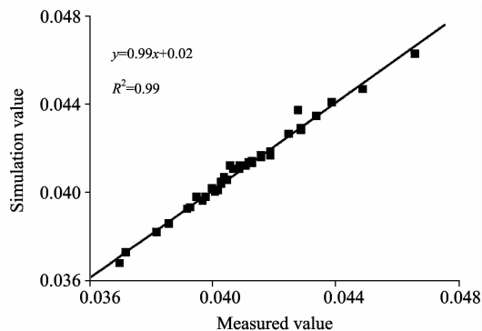
Fig. 2 Scatter plots of measured value versus simulation value for AM
