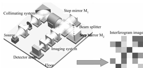
Fig. 1 Instrumental configuration of the static FTS
