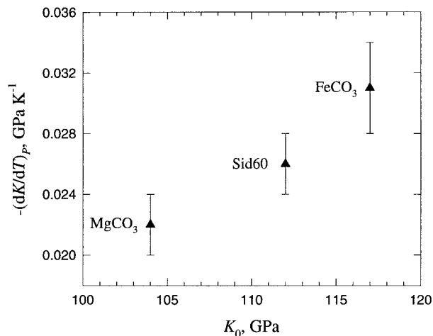
FIGURE 6. Relationship between the room-temperature bulk modulus and its temperature derivative. For MgCO 3 (magnesite), the value of (\partial K_T/\partial T)_p is from Zhang et al. (1997).
