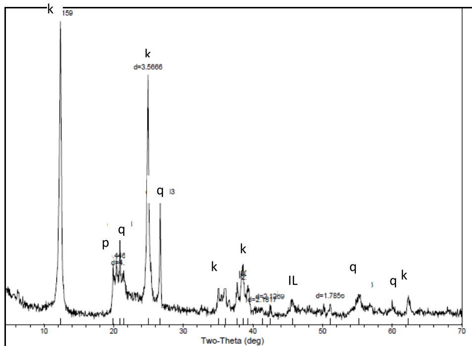
Fig. 6: X-ray diffractogram of Asaba sample 1 (k-kaolinite; q-quartz; p-palygorskite; IL-Illite)
