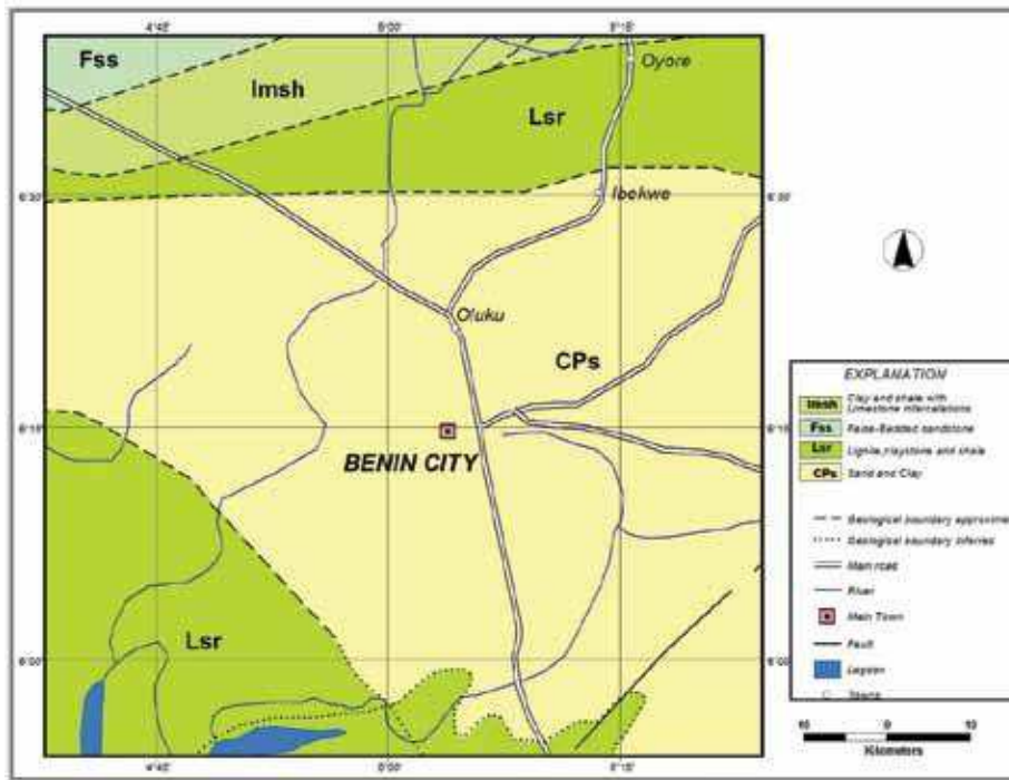
Fig. 5: Geological Map of Benin Area.
