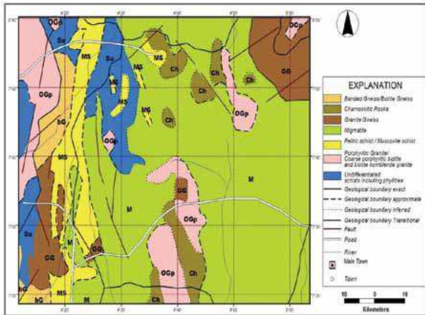
Fig 3. Geological map of Aramoko-Ekiti area
