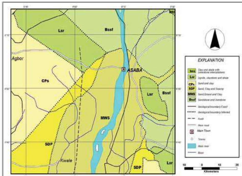
Fig. 2: Geological Map of Asaba Area
