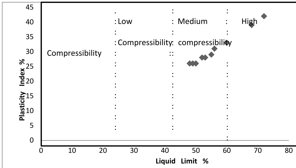
Fig 8: Relationship between Liquid limit and plasticity index for geophagic clays of Southern Nigeria (after Casagrande, 1948)
