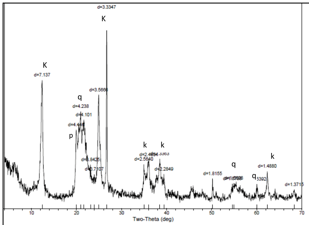
Fig. 7: X-ray diffractogram of Benin sample1(K – kaolinite; p – palygorskite; q – quartz;
