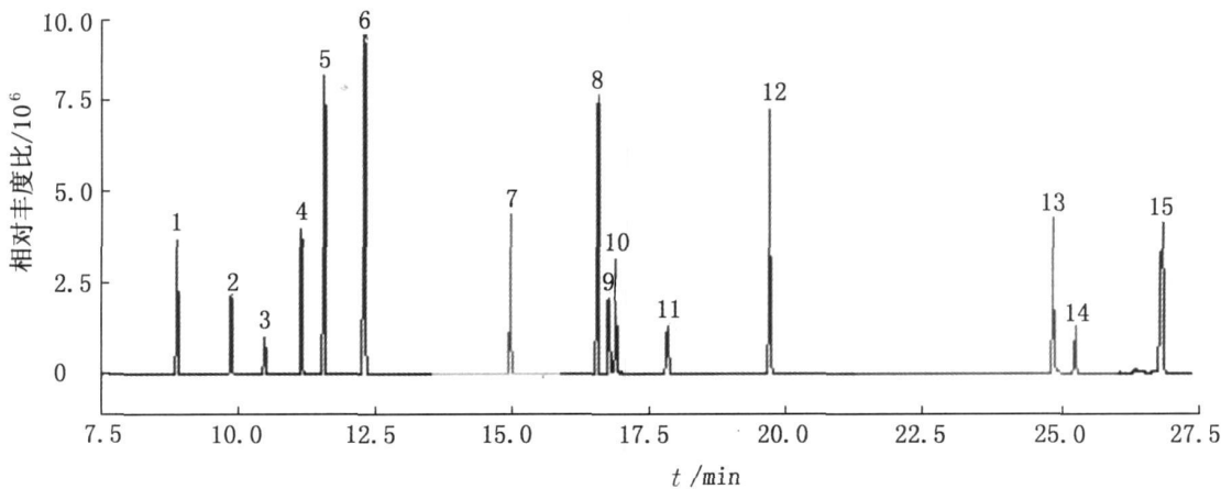
色谱峰: 1: \alpha - BHC; 2: \gamma - BHC; 3: \beta - BHC; 4: \delta - BHC; 5: 百菌清; 6: 三唑酮; 7: P, P- DDE; 8: 烯唑醇; 9: P, P- DDD; 10: O, P- DDT; 11: P, P- DDT; 12: 甲氰菊酯; 13: 氰戊菊酯 I; 14: 氰戊菊酯 II; 15: 溴氰菊酯(下图同)
