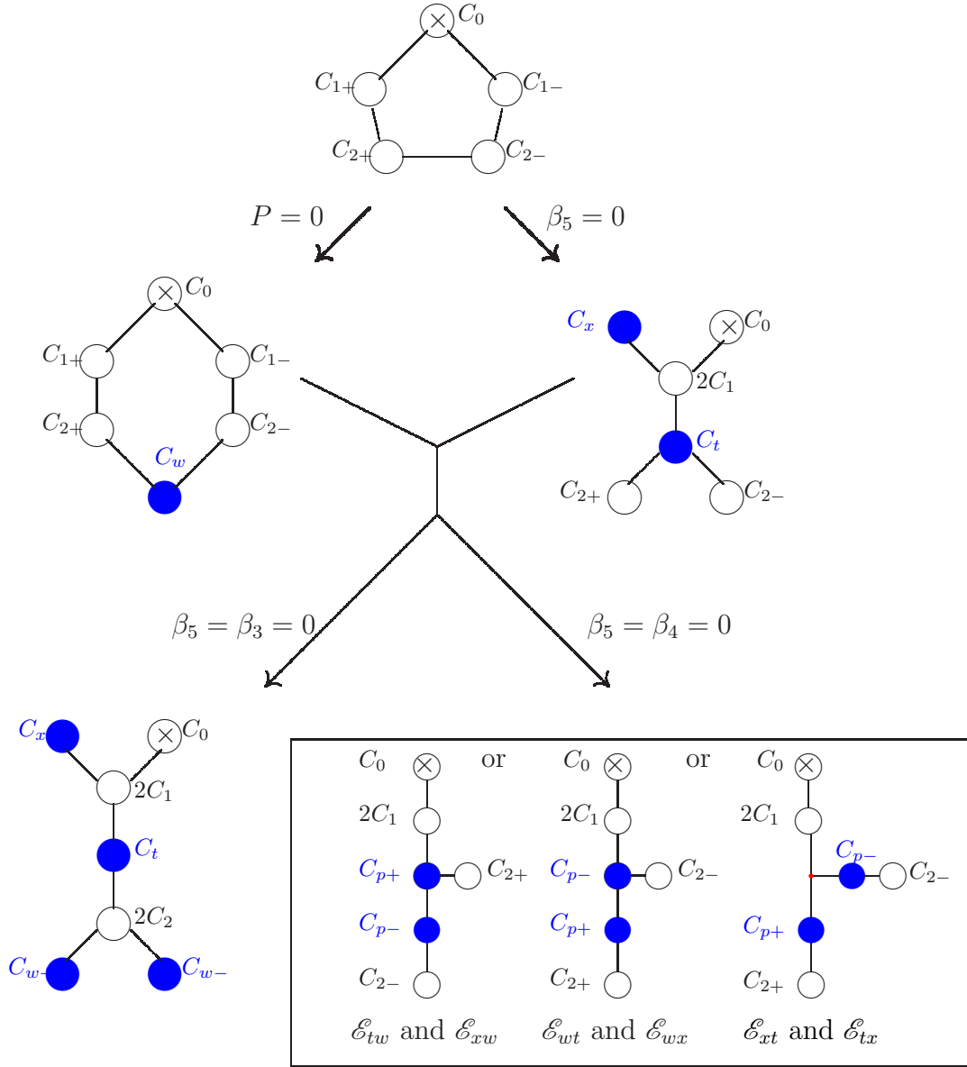
Figure 18: Fiber degeneration of an SU(5) GUTs with a small resolution. The nodes C_x , C_w and C_t are coming from the resolution of the higher codimensional singularities. We have 6 possible resolutions \mathcal{E}_{xw} , \mathcal{E}_{wx} , \mathcal{E}_{xt} , \mathcal{E}_{tw} and \mathcal{E}_{wt} . They are all related to each other by flop transitions related to permutation group of 3 elements.
