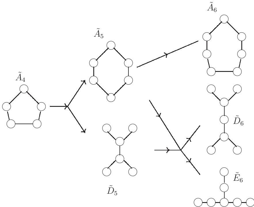
Figure 2: Conjectured singular fiber enhancements of a SU(5) GUT. Starting with codimension 1 in the base, the codimension increases from left to right. Thinking in terms of the dual graph, the rank of the associated Dynkin diagram increases by 1 as we move in codimension.
