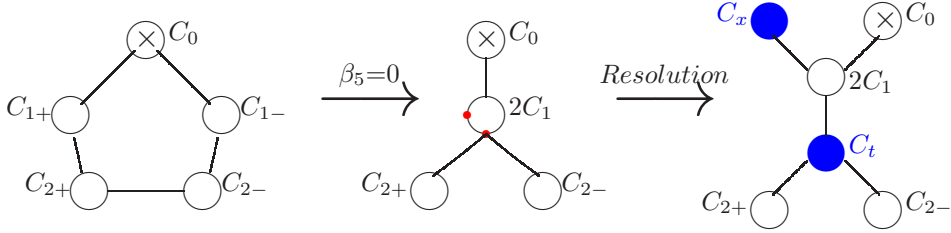
Figure 13: The codimension-2 fiber enhancement \tilde{A}_4 \rightarrow \tilde{D}_5 . It corresponds to the resolution of codimension-2 singularities above the curve w = \beta_5 = 0 . Although the new fiber is of type \tilde{D}_5 it does not correspond to a Kodaira fiber I_1^* since the node C_t (which is defined by a quadric equation) has multiplicity 1 and not 2.
