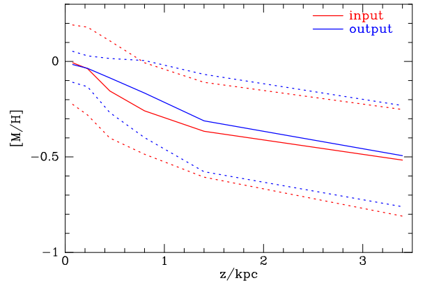
Fig. 15. The variation in the metallicity distribution as one moves away from the plane. Red: observed metallicities, blue: output metallicities. The solid line represents the median of each distribution and dashed lines show 1\sigma variations from the median.
