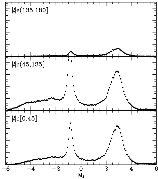
Fig. 9. The distribution of derived absolute magnitudes in ranges of Galactic longitude ( l ). The same vertical scale is used for all three panels so one gets an impression of the longitude-distribution of the entire sample.
