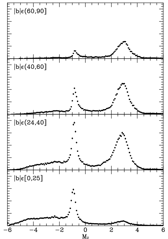
Fig. 8. The distribution of derived absolute magnitudes in slices of Galactic latitude ( |b| ). The same vertical scale is used for all four panels so one gets an impression of the latitude-distribution of the entire sample.
