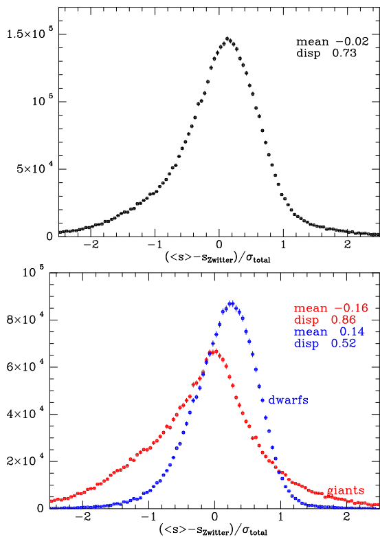
Fig. 6. Comparison of our results with those of Zwitter et al. (2010). Top panel: all 215 167 stars with two distances; lower panel: stars with \log g \geq 3.5 or < 3.5 grouped separately. The statistical uncertainties can be seen to be smaller than some of the points.
