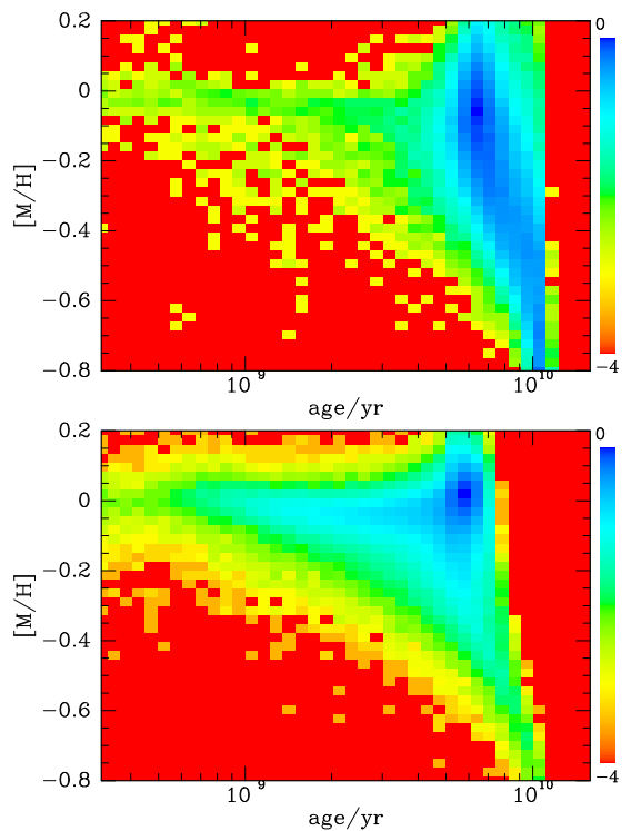
Fig. 18. The distribution of stars in the age–metallicity plane at |z| > 500 pc (above) and |z| < 500 pc (below). The colour encodes the base-10 logarithm of stellar density, with red indicating a complete absence of stars. The values of [M/H] used are the outputs of the distance-finding algorithm.
