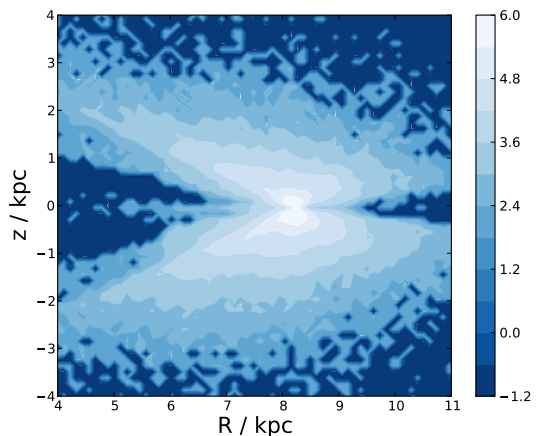
Fig. 12. The distribution of observed stars in the (R, z) plane. Contours are logarithmically spaced and represent densities in \log(\text{stars kpc}^{-2}) .
