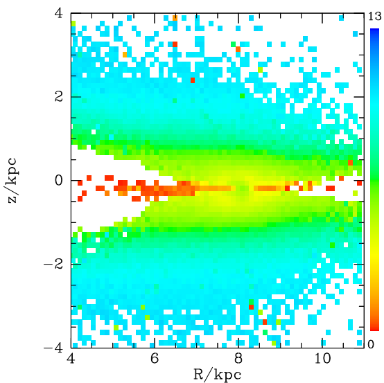
Fig. 16. The distribution of average stellar age in the (R, z) plane. The colour scale gives ages in Gyr. Regions for which there is inadequate data are white.
