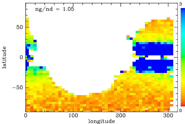
Fig. 10. The variation across the sky of the giant/dwarf fraction, with giants defined by \langle M_J \rangle < 1 and dwarfs by \langle M_J \rangle \geq 1 . White regions are not sampled by RAVE.
