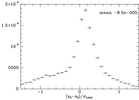
Fig. 5. The distribution for 15 525 stars with 3.3 < \log g < 3.7 of the differences s_{\text{VDR2}} - s_{\text{VDR3}} normalised by the quadrature sum of the formal errors.
