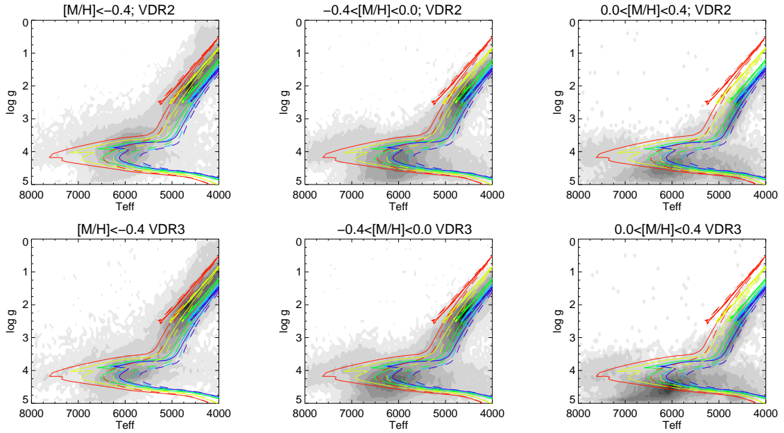
Fig. 2. The density of RAVE stars with S/N \geq 20 in the (T_{\text{eff}}, \log g) plane together with Padova isochrones for ages 3 Gyr (solid) and 9 Gyr (dashed). The colours indicate calibrated metallicities: [M/H] = -1 red; [M/H] = -0.6 yellow; [M/H] = -0.2 green; [M/H] = 0 light blue; [M/H] = 0.1 dark blue. The top row shows parameters from the VDR2 pipeline, while the lower row is for the VDR3 pipeline. In each row stars are grouped by metallicity, with the highest metallicities on the right. Note that in several panels, in the temperature range 6000 \leq T_{\text{eff}} \leq 7000 the density of stars is high below the lowest isochrone. This anomaly is most pronounced in the lower row.
