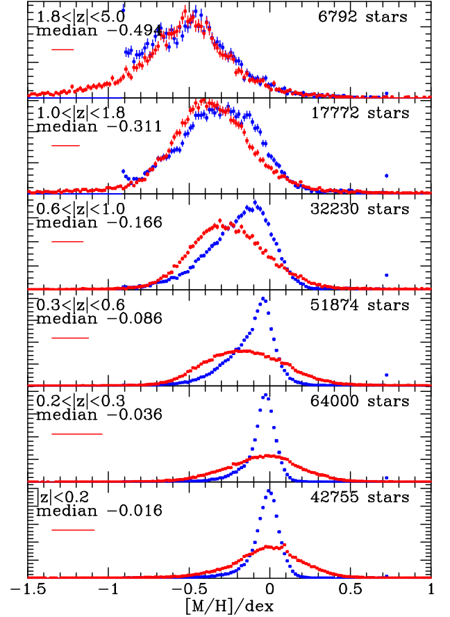
Fig. 14. The distribution in metallicity at several distance from the Galactic plane. Red points show observed metallicities, blue points show the output from our analysis. Values of |z| are in kpc, and the median output metallicity for each slice is displayed. The red scale bar in each panel represents the median observational error for that subsample.
