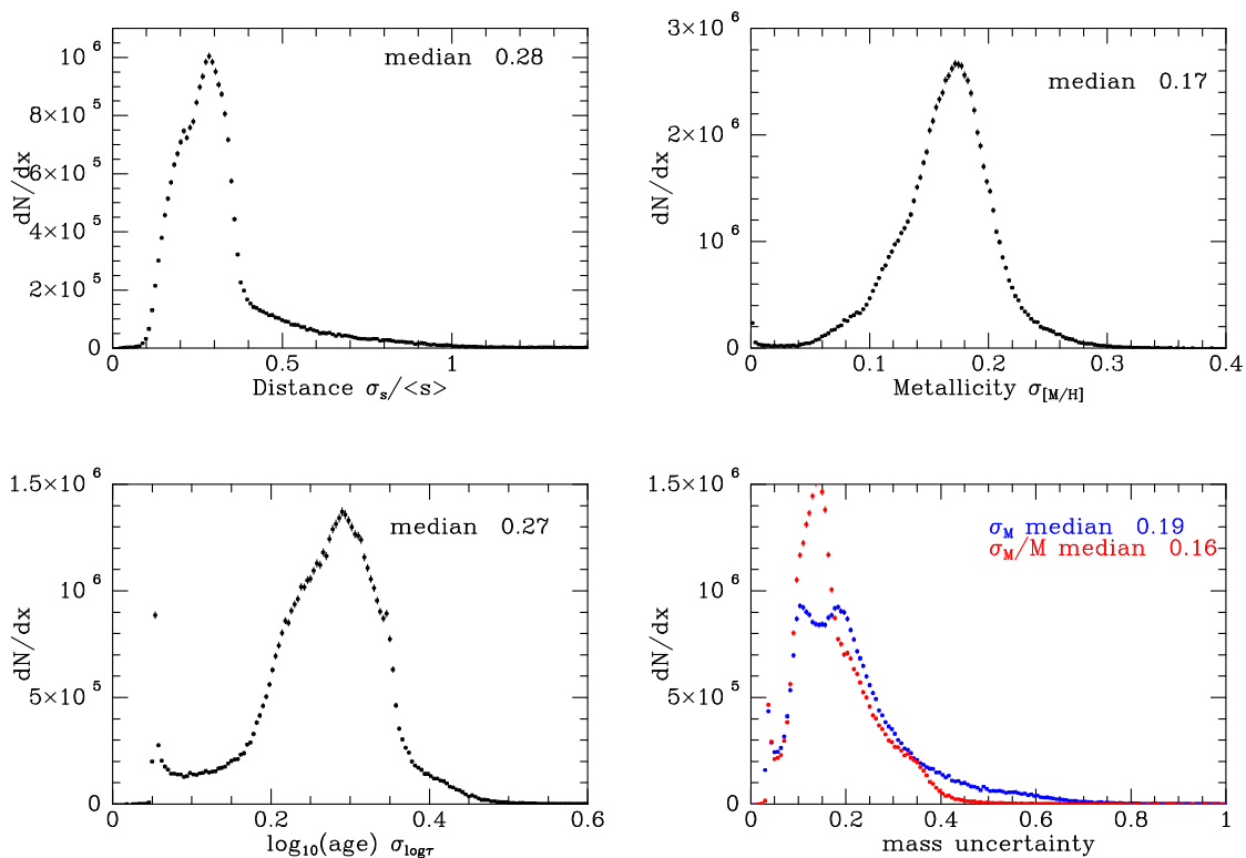
Fig. 7. Distributions of output errors for all four stellar parameters: distance s (top left); metallicity (top right); age (lower left); mass (lower right).
