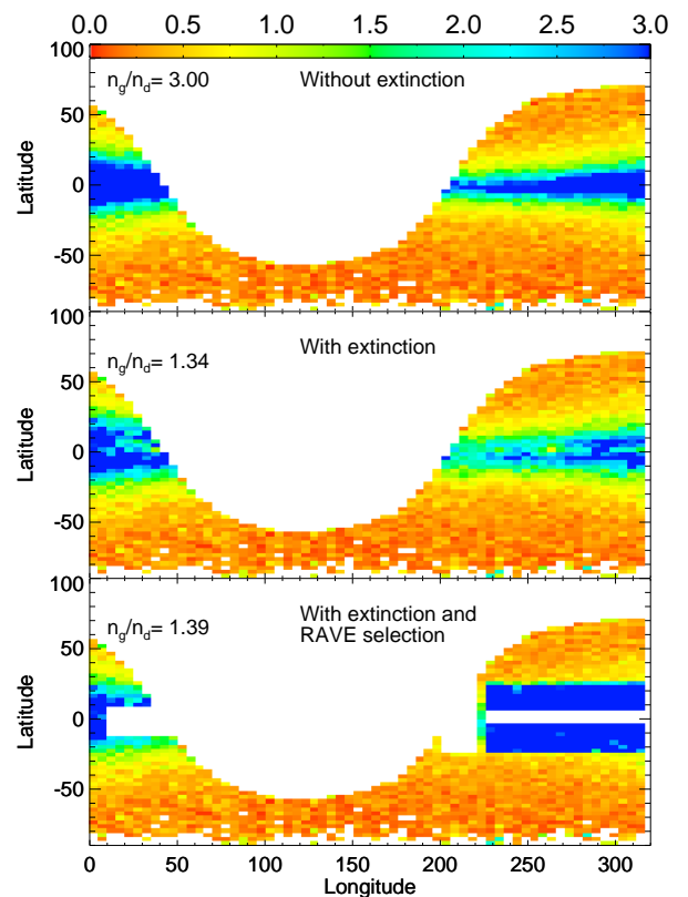
Fig. 11. The prediction of the Galaxy modelling code Galaxia (Sharma et al. 2011) for the structure of Fig. 10. The top two panels show all stars with 9 < l < 12 , without (top) and with (middle) including Galactic extinction. In the bottom panel low-latitude fields have been excluded and for 225^\circ < l < 315^\circ only stars with J - K > 0.5 are included.
