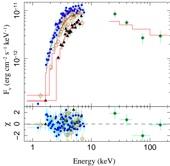
FIG. 3.— Spectral model of Table 1.
