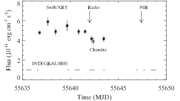
FIG. 1.— IGR J17177–3656 Swift and Chandra (absorbed) flux evolution in the 2–8 keV range. For clarity the INTEGRAL coverage of the source is also shown, marked as horizontal lines, together with our NIR and radio follow-up observations, as discussed in this paper.
