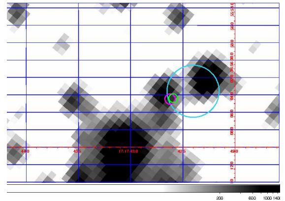
FIG. 7.— Final averaged K_s image of the field of view around IGR J17177–3656. As in Fig. 6, the green circle represents the ATCA position, the purple circle is the Chandra error, while the light-blue one is obtained with Swift .
