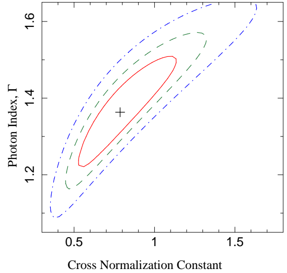
FIG. 4.— Contours of IBIS/ISGRI normalization constant vs. photon index. (68%, 90%, and 99% confidence for two parameters).
