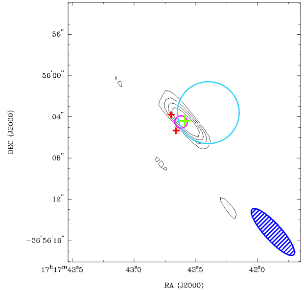
FIG. 6.— Radio map using the combined ATCA observations of IGR J17177–3656 at 5.5 and 9 GHz (see text). The green cross represents the fitted position of the ATCA counterpart, the purple circle is the 0.6'' Chandra error, the light-blue one the 3'' Swift error, while the red crosses are the two NIR candidates discussed in the text (Torres et al. 2011; Rojas et al. 2011).
