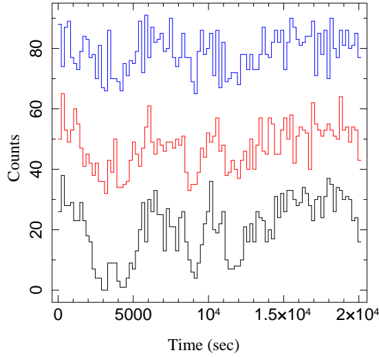
FIG. 2.— 200 s light-curves in 3 energy bands: 2–3.7 keV (black), 3.7–4.7 keV (red) and 4.7–8 keV (blue). For visualization purposes, the middle (red) and high band (blue) are offset by 30 and 60 counts with respect to the low (black) band.
