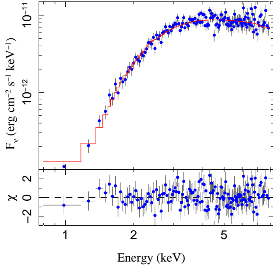
FIG. 5.— Swift average spectrum of IGR J17177–3656. See text for details.
