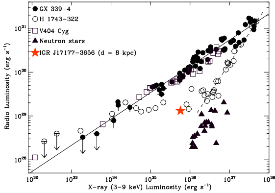
FIG. 8.— Radio to X-ray luminosity for a sample of black hole and neutron star LMXBs. Adapted from Coriat et al. (2011), see text for details.
