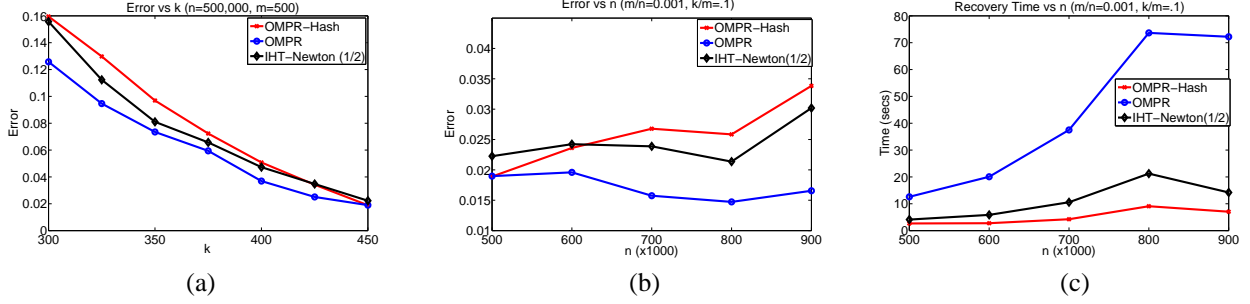
Figure 3: (a): Error ( \|Ax - b\| ) incurred by various methods as k increases. The measurements b = Ax are computing by generating x with support size m/10 . (b),(c): Error incurred and time required by various methods to recover vectors of support size 0.1m as n increases. IHT-Newton(1/2) refers to the IHT-Newton method with step size \eta = 1/2 .
