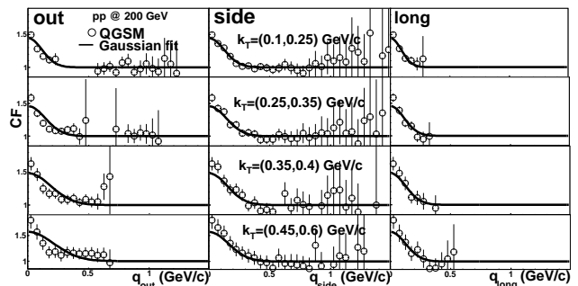
FIG. 11: Projections of the 3D Cartesian representations of the correlation functions onto the q_{out} , q_{side} , and q_{long} axes, for the minimum bias events from pp collisions at 200 GeV for four k_T ranges. To project onto one q -component, the others are integrated over the range 0 \leq q_i \leq 0.12 GeV/c.
