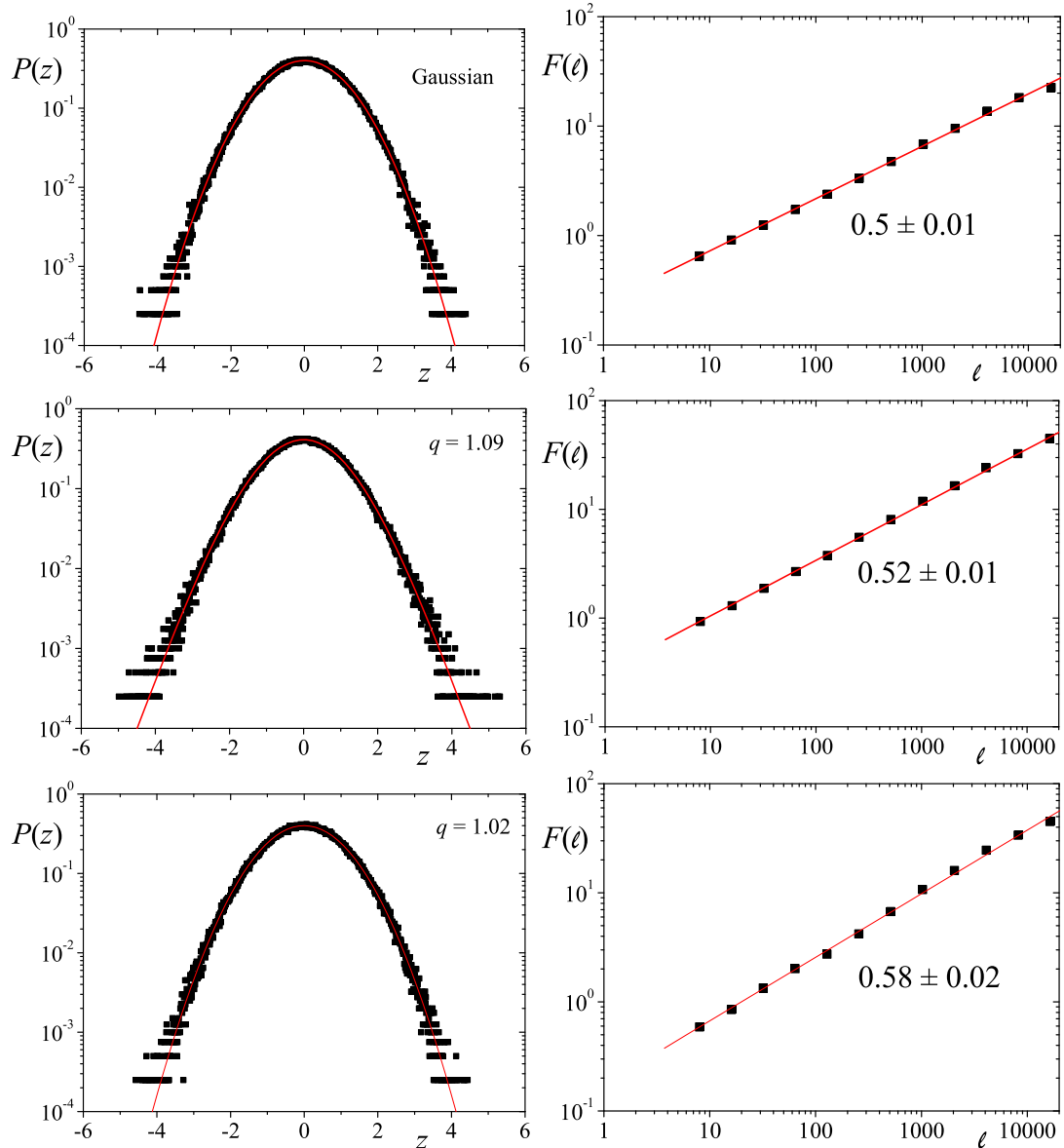
Figure 1: Left column: Probability density functions P(z) vs z in a log-linear scale; Right column: Fluctuation function F(\ell) vs \ell for |z| in a log-log scale. The values of the model parameters are: \phi = 0.1, W = 5 yielding q = 1 and H = 0.5 \pm 0.01 (upper panels); \phi = 5, W = 5 yielding q = 1.09 \pm 0.01 and H = 0.52 \pm 0.01 (middle panels); \phi = 2, W = 75 yielding q = 1.02 \pm 0.01 and H = 0.58 \pm 0.02 (lower panels). The results have been obtained from series of 4 \times 10^5 elements and the numerical adjustment of P(z) gave values of \chi^2/n never greater than 0.00003, with R never smaller than 0.998.
