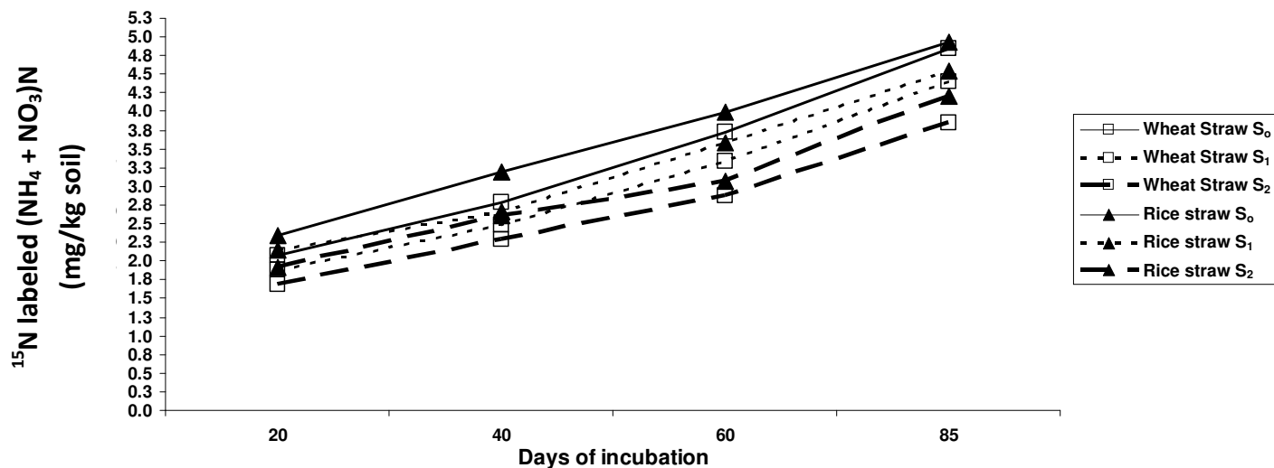
Figure 1. Mineralization of Nitrogen from ^{15}\text{N} labeled crop residues under varying clay content. S 0 , S 1 , S 2 refer to original soil, 75% original soil + 25% sand and 50% original soil + 50% sand respectively.
