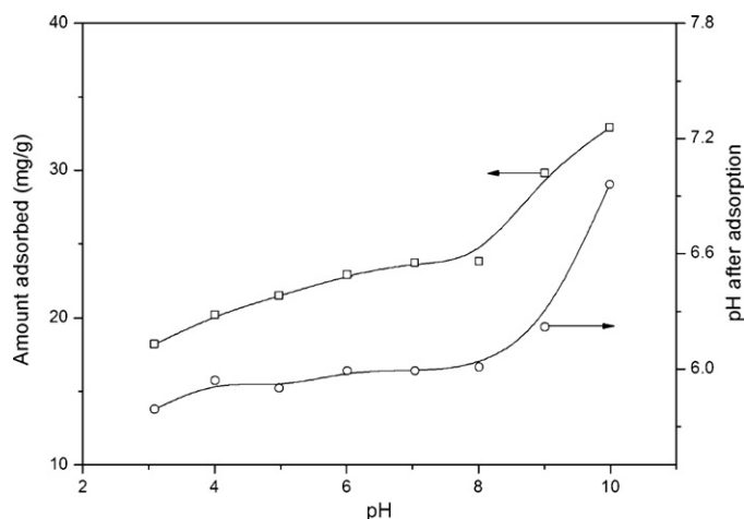
Fig. 2. Effect of pH on the adsorption capacity of \text{NH}_4^+\text{-N} onto CTS-g-PAA/APT (10 wt.%) ( T = 30\text{ }^{\circ}\text{C} , t = 4\text{ h} , C_0 = 100\text{ mg/L} , adsorbent dose = 50 mg/25 mL, 120 rpm).
