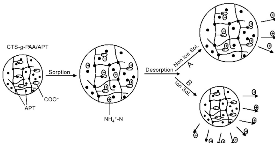
Fig. 6. Model scheme for the adsorption/desorption of \text{NH}_4^+\text{-N} onto/from CTS-g-PAA/APT polymeric networks. Non-ion sol., distilled water; Ion sol., 0.1 mol/L HCl (NaOH or NaCl); A, \text{NH}_4^+\text{-N} release of three-dimensional network adsorption; B, \text{NH}_4^+\text{-N} release of electrostatic adsorption.
