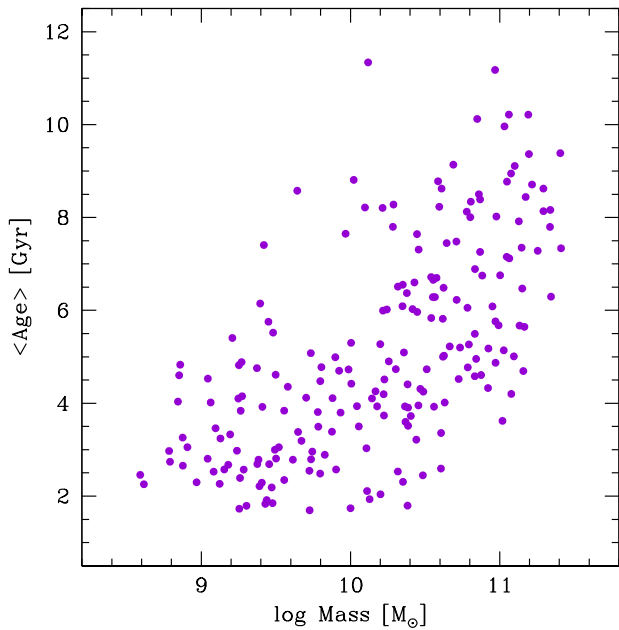
FIG. 3.— Mass-weighted average age as a function of the stellar mass for our host galaxies. As one would expect, the more massive galaxies tend to be the older galaxies, though the scatter in the relation is large.
