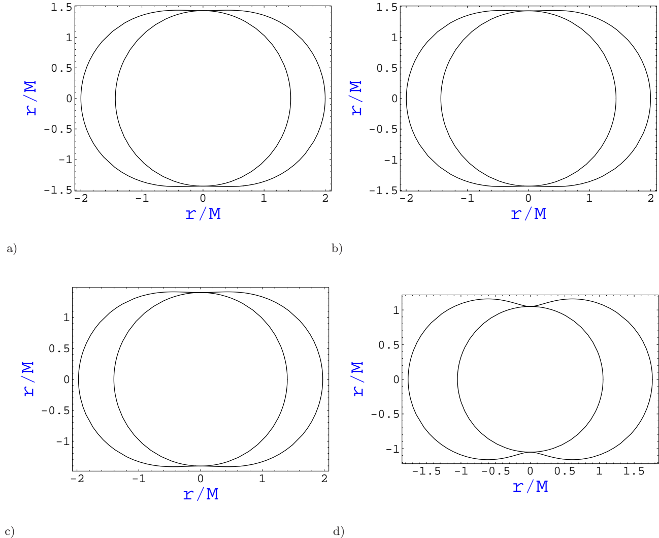
FIG. 1: The dependence of the shape of the ergosphere from the small dimensionless parameter \delta : a) \delta = 0 , b) \delta = 0.001 c) \delta = 0.01 , d) \delta = 0.1 .
