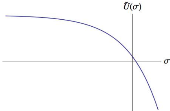
FIG. 1. Plot of the Einstein-frame potential \tilde{U}(\sigma) .
