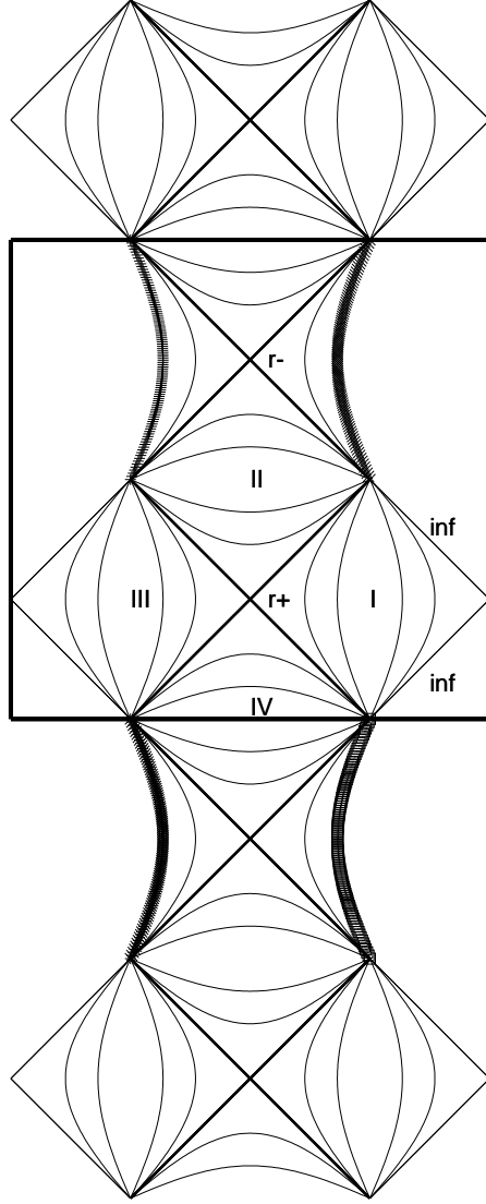
Fig. 1 The conformal diagram of the maximally extended Reissner–Nordström spacetime with \Lambda = 0 and e^2 < m^2 . It can either be interpreted as an infinite chain of copies of the segment within the rectangle, or one can identify the upper side of the rectangle with the lower side, obtaining a manifold with closed timelike and null lines. More explanation in the text.
