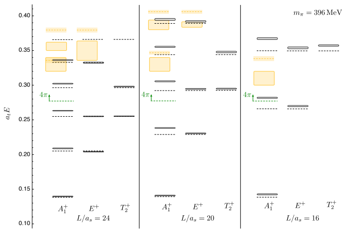
FIG. 1: Low-lying spectrum, in units of the temporal lattice spacing, of finite volume states in irreps A_1^+, E^+, T_2^+ at m_\pi = 396 MeV for L/a_s = 16, 20, 24 . The box size indicates the statistical uncertainty on the energy. Orange boxes correspond to states suspected of being \pi\pi^* scattering states. Dashed lines indicate the non-interacting energy of pion pairs with the allowed lattice momenta between them.
