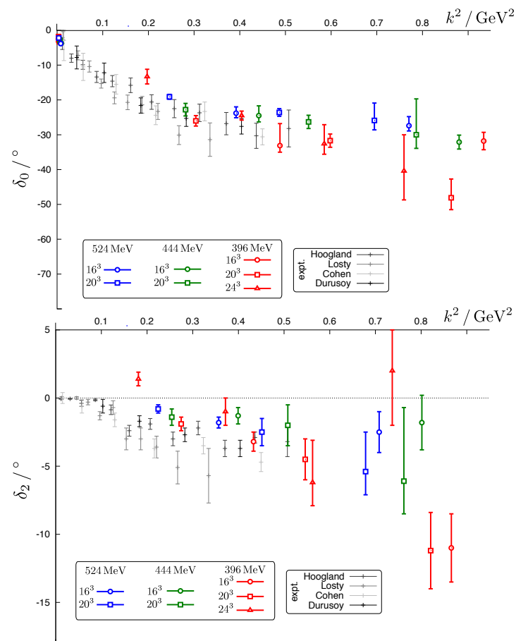
FIG. 3: Phase-shift in degrees for \pi\pi I = 2 scattering with \ell = 0 ( \delta_0 ) and \ell = 2 ( \delta_2 ). Lattice results at various pion masses and volumes. Experimental data from [7–10].
