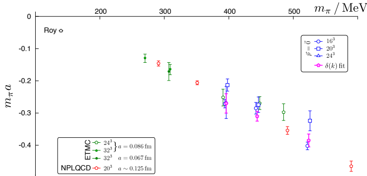
FIG. 4: S -wave scattering length. Blue points from \vec{p} = \vec{0} correlators, pink points from effective range fits to \delta(k) . Comparison to lattice results of [4, 5] and Roy equations analysis of experimental data [15].
