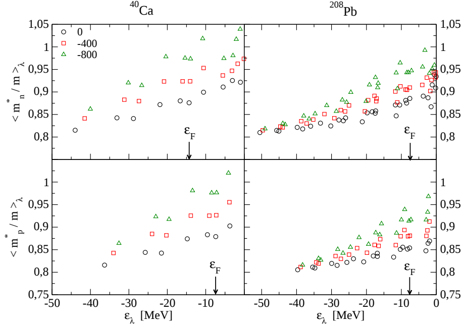
Figure 2: Energy dependence of the expectation value of \langle m_q^*/m \rangle_\lambda for bound states for ^{40}\text{Ca} and ^{208}\text{Pb} , for C_0^{\tau(\nabla\rho)^2} = 0, -400, -800 \text{ MeV fm}^{10} . The arrows indicate the position of the Fermi energy for C_0^{\tau(\nabla\rho)^2} = 0 \text{ MeV fm}^{10} defined as the energy of the last occupied state. The correction induced by the surface-peaked effective mass produces an increase of the Fermi energy by 400 keV at most.
