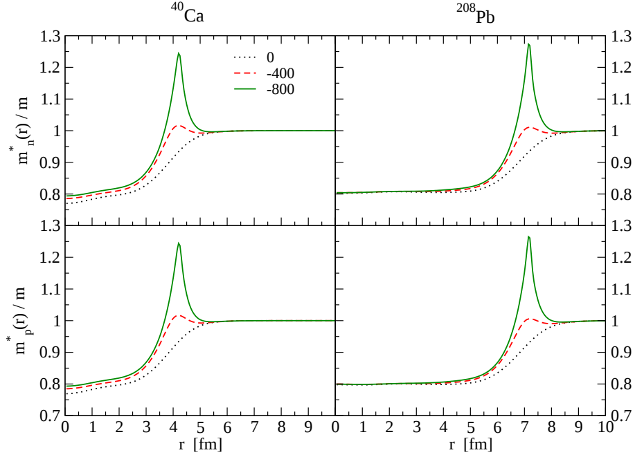
Figure 1: m_q^*/m as a function of radial coordinate for ^{40}\text{Ca} and ^{208}\text{Pb} , for C_0^{\tau(\nabla\rho)^2} = 0, -400, -800 MeV fm 10 .
