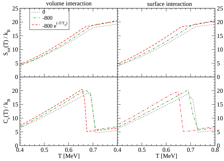
Figure 10: Total entropy S_{tot} and specific heat C_V (in units of the Boltzmann constant), for ^{120}\text{Sn} as a function of temperature, for C_0^{\tau(\nabla\rho)^2} = 0 , -800 MeV fm 10 , -800 e^{-T/T_0} MeV fm 10 , and for volume (on the left) and surface (on the right) pairing interaction.
