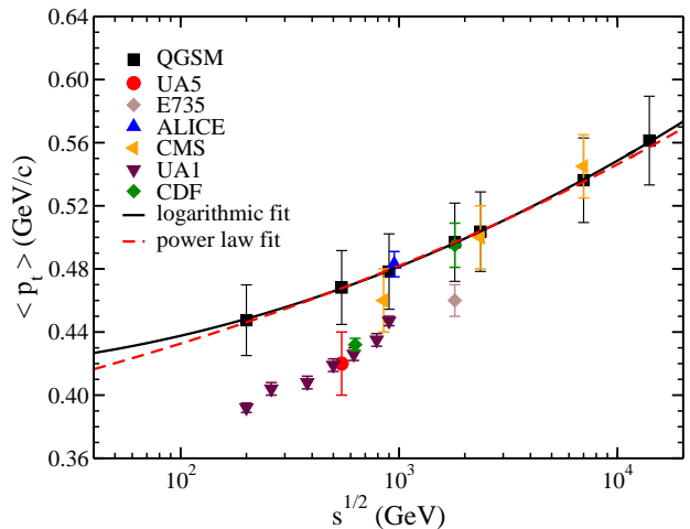
FIG. 4: (Color online) Average transverse momentum as function of \sqrt{s} . Squares present the QGSM results, other symbols denote experimental data from [42–45, 48, 50]. Solid and dashed lines are fit to logarithmic and power-law dependences, respectively. See text for details.
