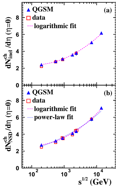
FIG. 7: (Color online) The charged particle density at midrapidity as a function of \sqrt{s} for (a) inelastic and (b) non-single diffractive collisions. Dashed lines show the results of the fit to expression a + b \ln s + c \ln^2 s , dotted line (b) - to the power-law dependence d\sqrt{s}^\lambda .
