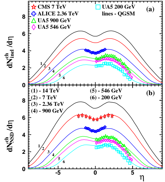
FIG. 6: (Color online) The charged particle pseudorapidity spectra for (a) inelastic and (b) non-single-diffractive events calculated in QGSM for pp collisions at \sqrt{s} = 200 GeV (6), 546 GeV (5), 900 GeV (4), 2.36 TeV (3), 7 TeV (2) and 14 TeV (1). Data are taken from [42, 47, 50].
