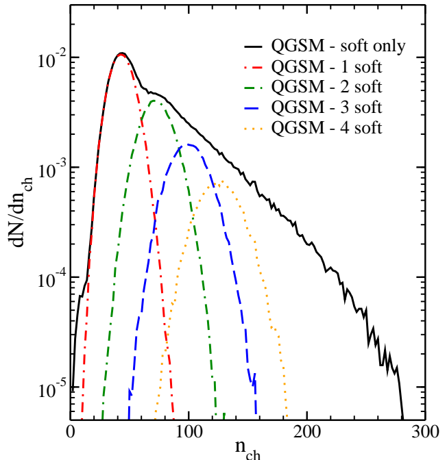
FIG. 12: (Color online) Charged-particle multiplicity distribution (solid line) for processes going via the exchange of n \geq 1 soft Pomerons in pp collisions at \sqrt{s} = 14 TeV. Contributions of first four terms are shown by dash-dotted ( n = 1 ), double-dash-dotted ( n = 2 ), dashed ( n = 3 ) and dotted ( n = 4 ) lines, respectively.
