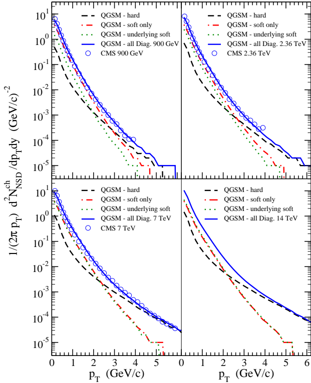
FIG. 5: (Color online) Transverse momentum distributions of the invariant cross section of charged particles in NSD pp collisions at (a) \sqrt{s} = 900 GeV, (b) \sqrt{s} = 2360 GeV, (c) \sqrt{s} = 7 TeV and (d) \sqrt{s} = 14 TeV calculated in QGSM. Combined contribution of all processes and, separately, of only soft, hard and underlying soft sub-processes are shown by solid, dash-dotted, dashed and dotted lines, respectively (see text for details). Experimental data plotted in (a), (b) and (c) panels are taken from [49, 50].
