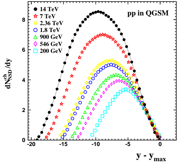
FIG. 8: (Color online) The distributions \frac{1}{\sigma_{NSD}} \frac{d\sigma_{NSD}}{dy} as functions of rapidity difference y - y_{max} obtained in QGSM for energies \sqrt{s} = 200 GeV, 546 GeV, 900 GeV, 1.8 TeV, 2.36 TeV, 7 TeV and 14 TeV.
