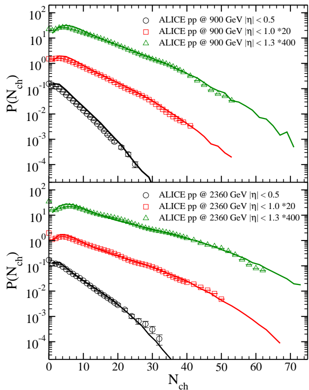
FIG. 10: (Color online) Charged-particle multiplicity distributions in |\eta| < 0.5 , |\eta| < 1.0 and |\eta| < 1.3 intervals, obtained in QGSM for pp collisions at \sqrt{s} = 900 GeV (upper plot) and at \sqrt{s} = 2360 GeV (bottom plot). Open symbols show the corresponding ALICE data [47].
