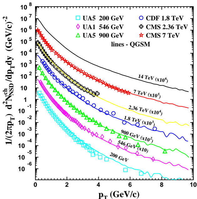
FIG. 3: (Color online) Transverse momentum distributions of the invariant cross section of charged particles in NSD pp collisions obtained in QGSM at |y| \leq 2.5 for all energies in question. Experimental data are taken from [42–44, 50].
