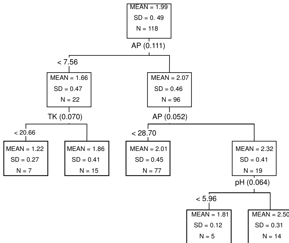
Figure 3. Regression tree predicting soybean yields from soil variables (PRE = 0.29). Each node (square) is labeled with average yield (Mean), standard deviation (S.D.) and the number (n) of fields in that group. The model is read from top down until terminal nodes appear. Partial PRE values are presented in parentheses at each root node to split.
