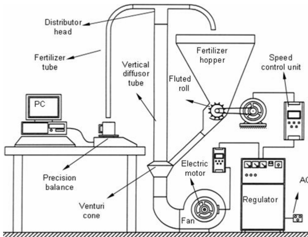
Figure 1. Measurement setup.
