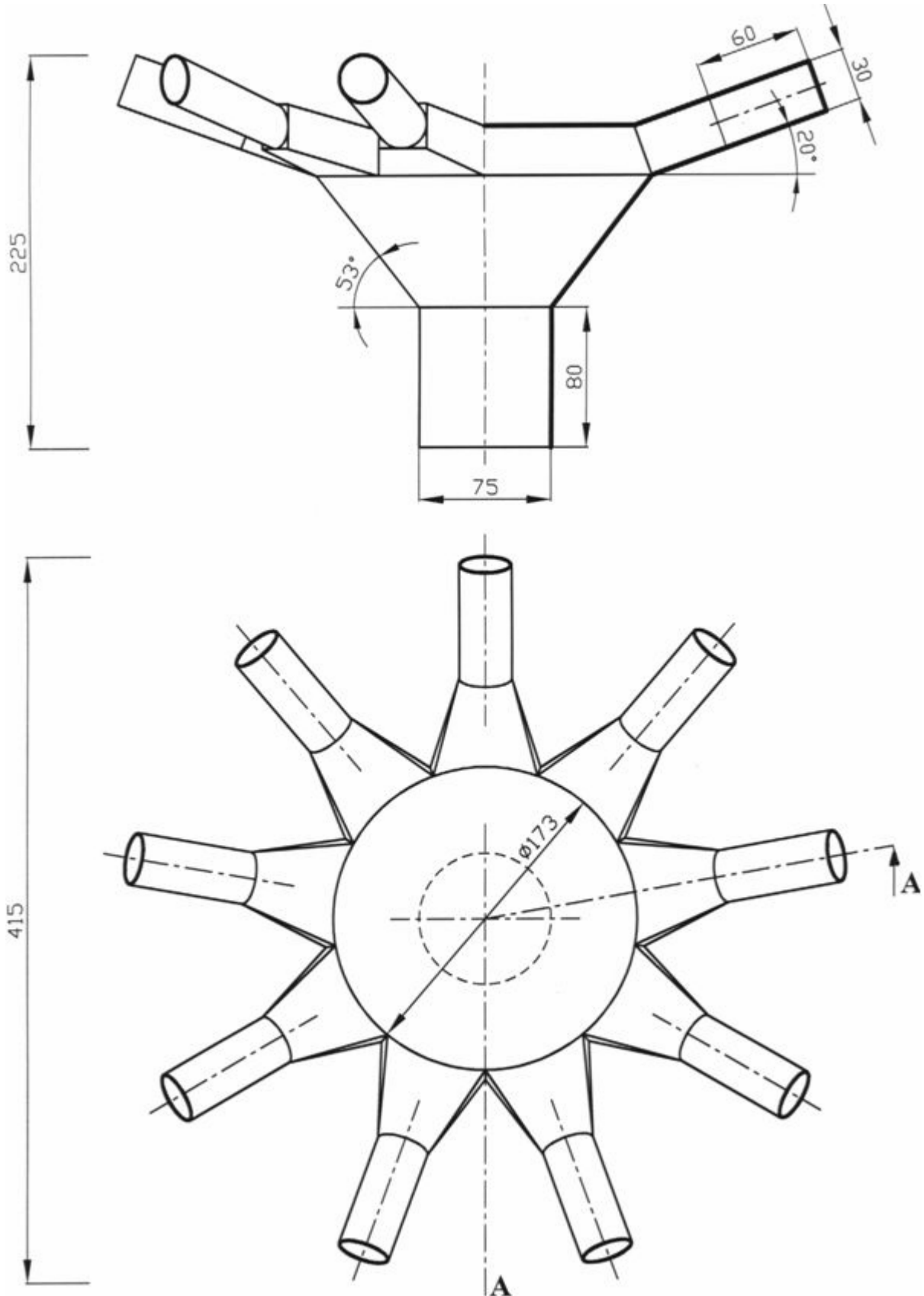
Figure 2b. Constructive properties of funnel distributor head.
