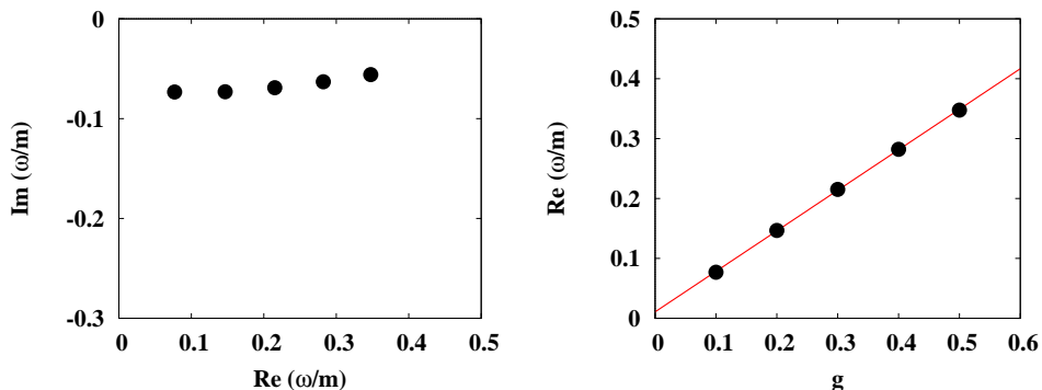
FIG. 6: The left panel shows the coupling constant dependence of the fermion pole with a particle number in the positive energy region for T/m = 2.0 and \alpha = 1.0 , at zero momentum: the horizontal and the vertical axis denote the real and imaginary part of the energy, respectively. The dots from left to right correspond to g = 0.1, 0.2, 0.3, 0.4, 0.5 , respectively. The right panel shows the coupling constant dependence of the real part of the fermion(particle) pole in the positive energy region at zero momentum for the same T/m and \alpha . The solid line is the fitted linear function.
