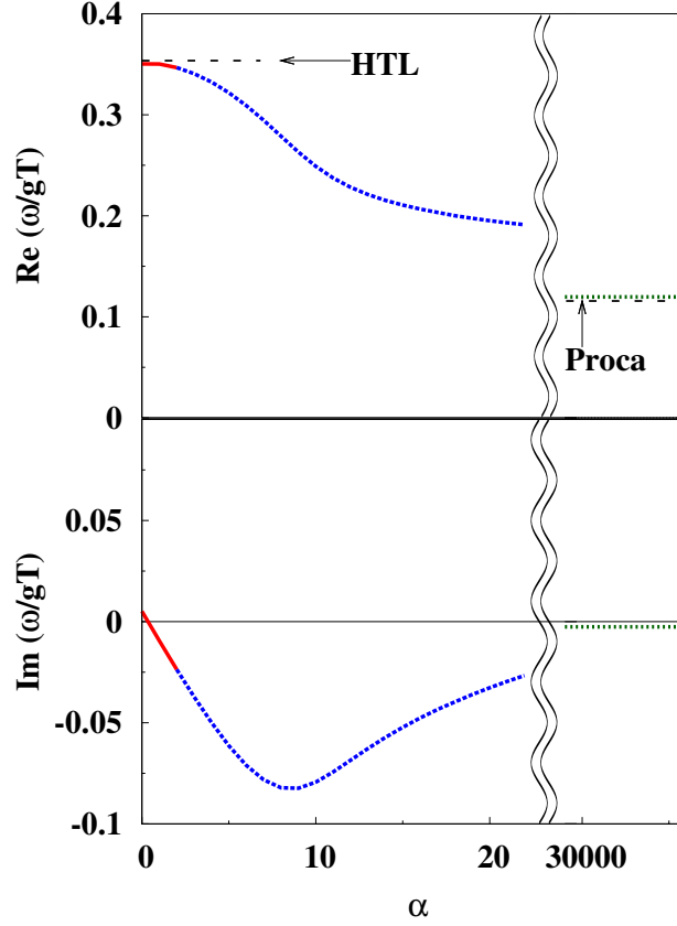
FIG. 10: The upper panel shows the gauge dependence of the real part of the pole in the positive energy region at zero momentum at T = 40.0m , for g = 0.5 . The horizontal and the vertical axes denote the gauge parameter \alpha and the real part of the pole, respectively. The data whose \alpha is smaller than the upper limit of adequate gauge parameter, 1/g = 2.0 , are denoted by the solid line and the data whose \alpha is larger than 1/g by the dotted line. The data which satisfy \alpha > 1/(g^2\lambda) = 1600 , which are expected to approach the value in the Proca formalism, are plotted with another dotted line. The upper and lower dashed lines show the thermal mass in the HTL approximation gT/(2\sqrt{2}) and that in the Proca formalism \sqrt{6m}/\sqrt{1+48\lambda} \simeq 2.31m , respectively. The lower panel shows the gauge dependence of the imaginary part of the pole for the same T and g as in the upper panel.
