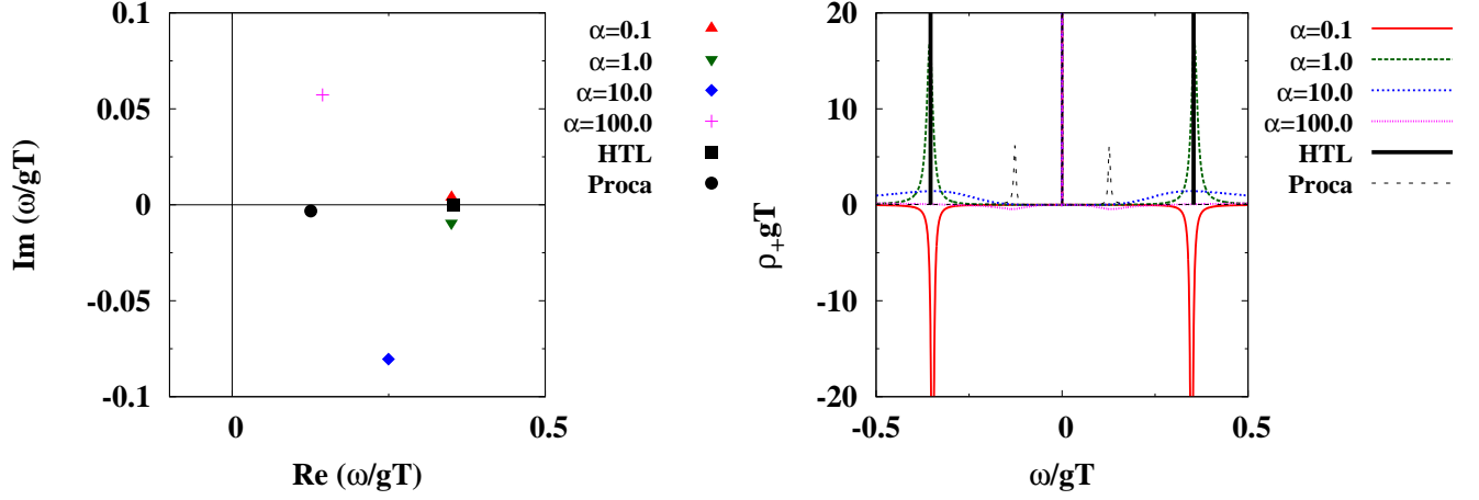
FIG. 8: The left panel shows the gauge dependence of the fermion pole at p = 0 in the positive energy region at T = 40.0m for g = 0.5 : The horizontal and the vertical axis denote the real and imaginary part of energy. The right panel shows the fermion spectral function in the particle sector \rho_+ as a function of energy \omega for the same T and g .
