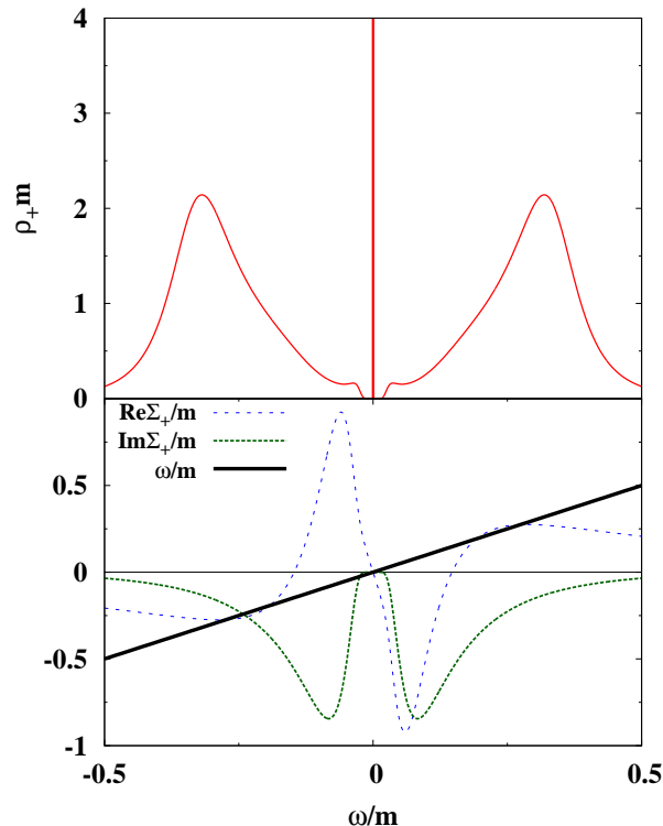
FIG. 7: The upper figure shows the fermion spectral function in the particle sector \rho_+ as a function of energy \omega for g = 0.5 , T = 2.0m , and \alpha = 1 . The lower figure shows the real part and the imaginary part of the fermion self-energy as functions of energy \omega for the same g , T , and \alpha . The dotted line denotes \omega . The intersection points between this line and \text{Re}\Sigma_+(\mathbf{0}, \omega) are the solutions of the dispersion relation.
