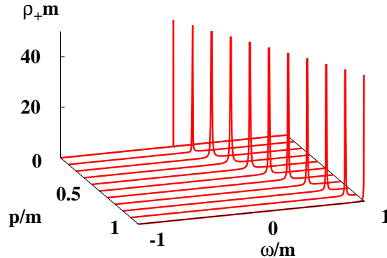
FIG. 2: The fermion spectral function in the particle sector \rho_+ as a function of energy \omega and momentum p for T = 0.4m , g = 0.5 , \alpha = 1 .
