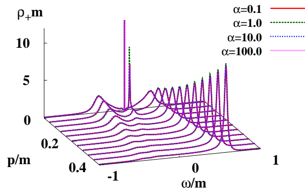
FIG. 4: The spectral fermion function in the particle sector \rho_+ as a function of energy \omega and momentum p at T = 2.0m , g = 0.5 .
