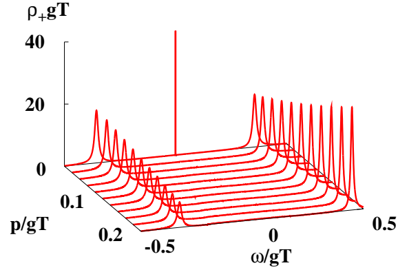
FIG. 9: The fermion spectral function in the particle sector \rho_+ as a function of energy \omega and momentum p at T = 40.0m with g = 0.5 and \alpha = 1 .
