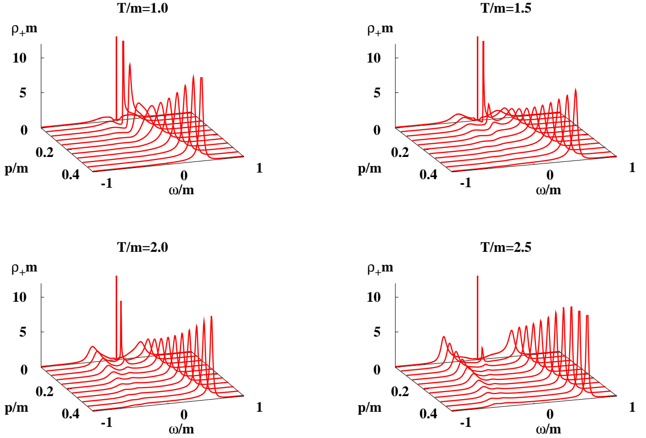
FIG. 3: The fermion spectral function in the particle sector \rho_+ as a function of energy \omega and momentum p at g = 0.5 , \alpha = 1 at various temperatures.
