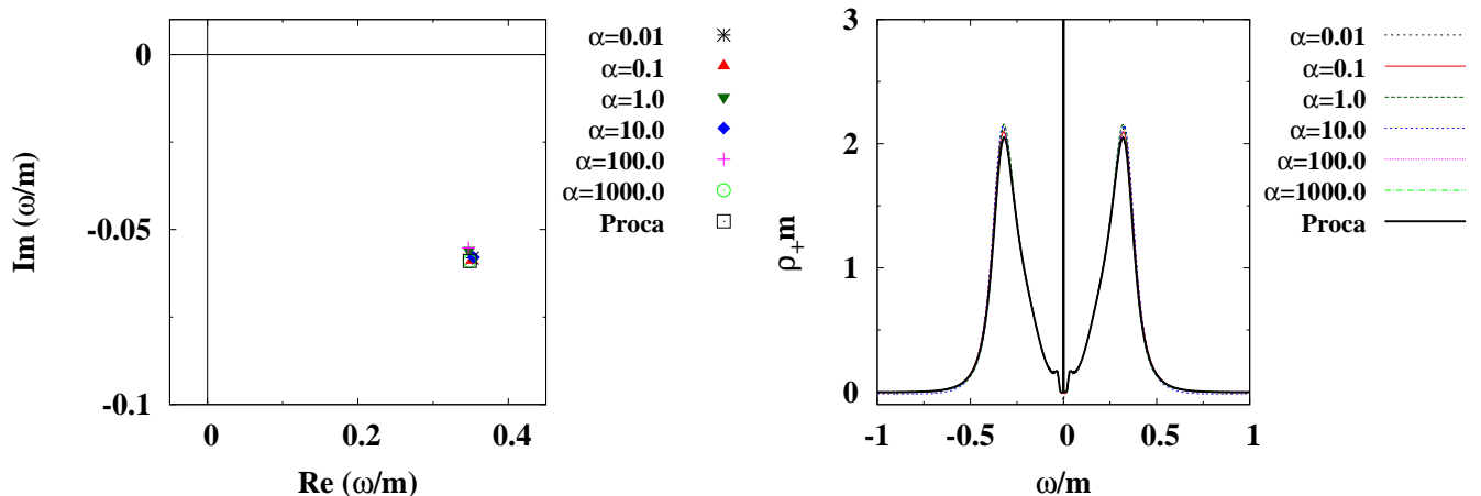
FIG. 5: The left panel shows the gauge dependence of the fermion pole with a positive particle number in the positive energy region for T = 2.0m , g = 0.5 at zero momentum: the horizontal and vertical axes denote the real and imaginary part of the energy, respectively. The right panel shows the fermion spectral function in the particle sector \rho_+ as a function of energy \omega for the same T, g as the left panel.
