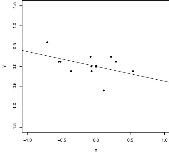
Figure 3. The plot whose slope = -K used to determine the Kuramoto coupling parameter. x are the values of \frac{\partial}{\partial \theta} [\rho \int_0^{2\pi} \sin(\theta' - \theta) \rho(\theta', t, 0) d\theta'] while y are the values of \omega \frac{\partial \rho}{\partial \theta}
