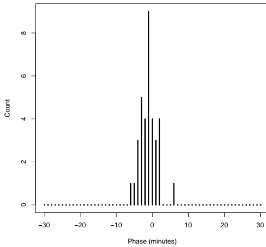
Figure 1. The count (not proportional) phase density plot of the measurements of watch time phase difference from the computer timestamp as measured in the experiment.
