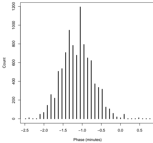
Figure 2. The distribution of the mean phase from a 1000 sample bootstrap.
