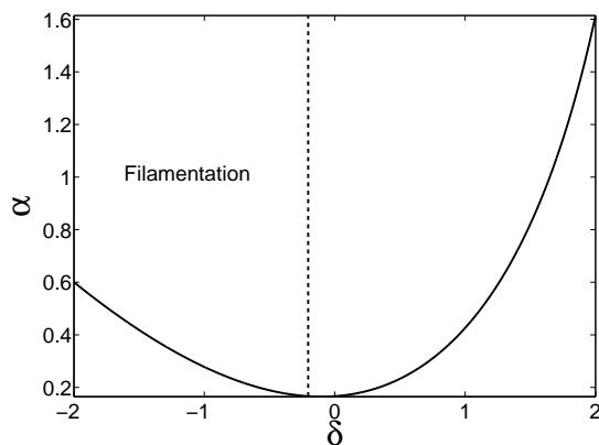
FIG. 5: Lossless SPPs exist above the full line corresponding to \alpha = \alpha_0 . SPPs are unstable with respect to filamentation on the left from the dashed vertical line, corresponding to \text{Re}\gamma = 0 . \lambda_a = 400 \text{ nm} .
