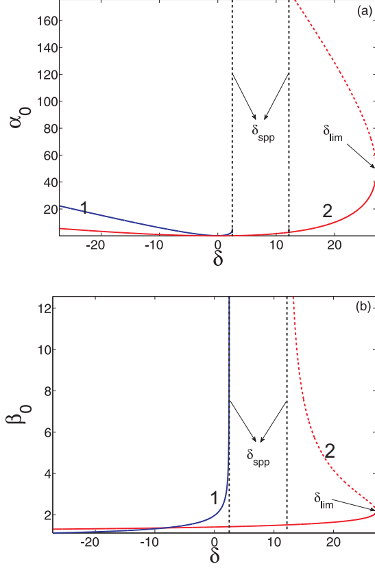
FIG. 1: (Color online) (a) Threshold gain \alpha_0 vs detuning \delta for two different atomic resonances: \lambda_a = 400\text{nm} (line 1 (blue)) and \lambda_a = 700\text{nm} (line 2 (red)). (b) \beta_0 vs \delta . Parameters and notations as in a). The full/dashed line corresponds to the minus/plus in Eq. (11).
