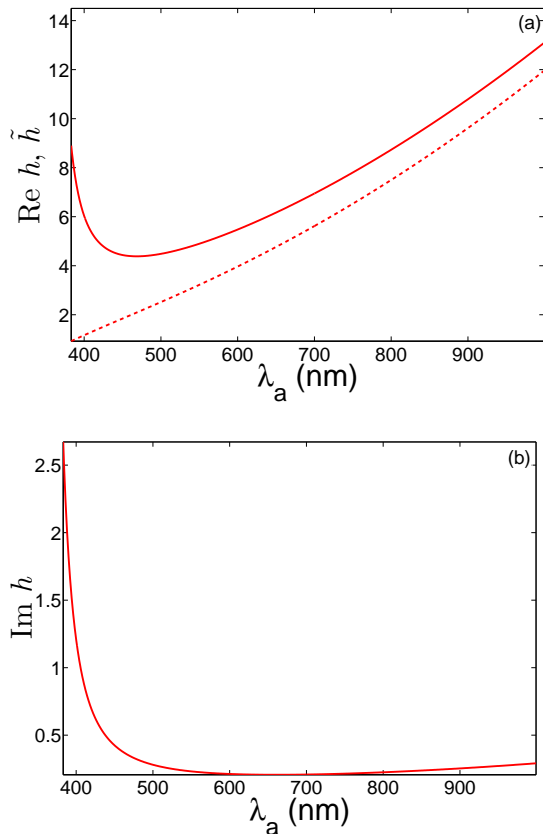
FIG. 2: (Color online) (a) Nonlinearity enhancement coefficients \text{Re}h (full line) and \tilde{h} (dashed line) calculated using two different approaches vs \lambda_a . (b) \text{Im}h . Varying \delta inside the transition linewidth leads only to small difference in h . The graphs shown correspond to \delta = -0.5 . The short wavelength boundary of the both plots corresponds to the point where \beta_0 becomes imaginary.
