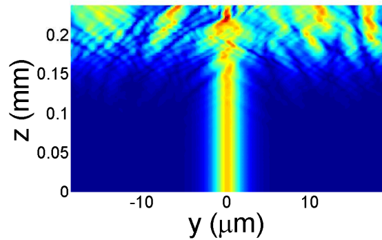
FIG. 6: (Color online) Propagation of a bright localized solution and instability of its background: \lambda_a = 594 \text{ nm} , \delta = -0.3 , \alpha = 0.0183 , \alpha_0 = 0.0063 .
