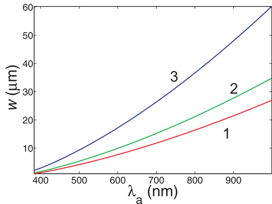
FIG. 4: (Color online) The characteristic filament size w scaled back into physical units vs \lambda_a for \delta = -0.5 , g = 0.1, 0.3, 0.5 for blue (line 3), green (line 2) and red (line 1) curves respectively.
