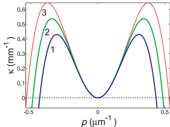
FIG. 3: (Color online) Growth rate \kappa of the filamentation instability expressed in physical units as a function of momentum p . \lambda_a = 594 \text{ nm} , \delta = -0.3 , \alpha_0 = 0.0063 and g = 0.4, 0.5, 0.6 for blue (line 1), green (line 2) and red (line 3) curves respectively.
