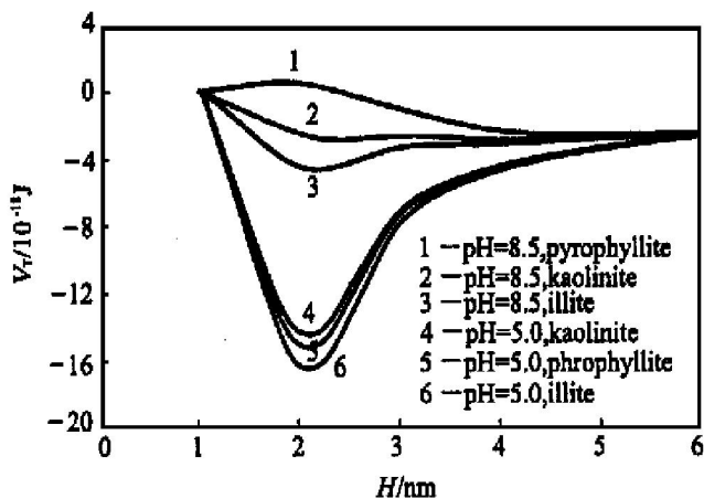
图3 一水硬铝石与含硅脉石矿物间的总相互作用能 Fig. 3 Total interaction between diaspore and silicate minerals
