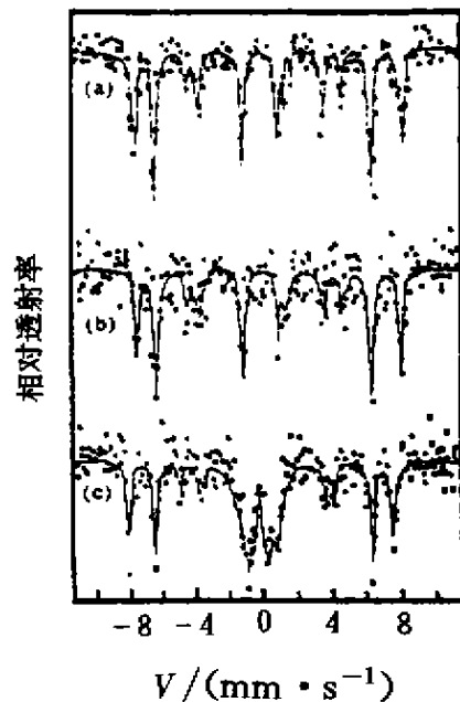
图 1 多晶钷铁石榴石的穆斯堡尔谱 (a)未辐照, (b) S_e = 2.9 MeV/ \mu m, (c) S_e = 5.8 MeV/ \mu m, (b)和(c)辐照剂量均为 5.0 \times 10^{14} Ar/cm 2 .
