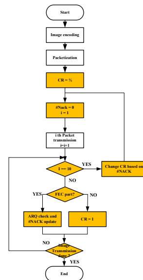
(a) Transmitter
