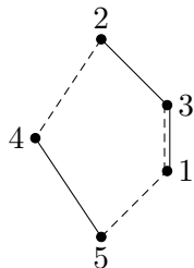
FIGURE 1. A non-messing-up poset P whose rows are drawn with dashed lines and columns with solid. A labeling \lambda of P is also given.
