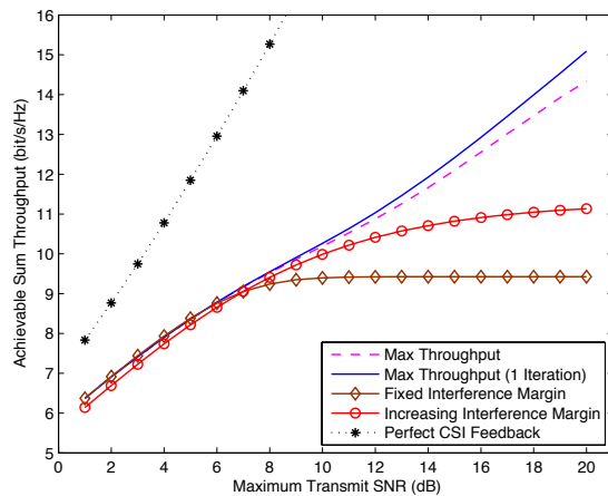
Fig. 2. Comparison of achievable sum throughput between different IPC feedback algorithms for the coupling factor \nu = 0.2 .
