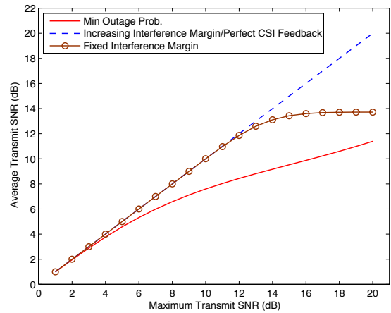
Fig. 3. Comparison of outage probability (upper) and average transmit SNR (lower) between different IPC feedback algorithms for the coupling factor \nu = 0.05 .
