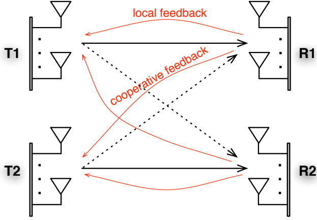
Fig. 1. MIMO interference channels with local and cooperative feedback.
