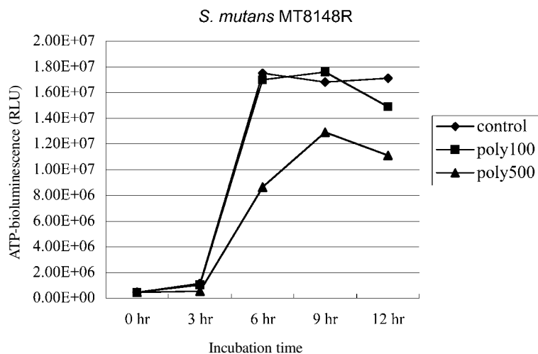
Fig. 2 Inhibitory effect of cranberry polyphenol on growth of S. mutans MT8148R. Poly 100, 500 mean cranberry polyphenol, 100 or 500 \mu g/ml, respectively.
