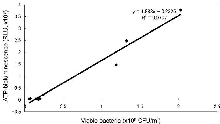
Fig. 1 Relationship between viable cell count (CFU) and ATP-bioluminescence
