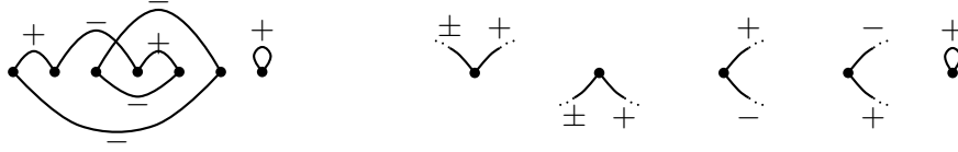
FIGURE 4. The signed arch diagram of \pi = 2, -4, -6, 5, -3, -1, 7 , and the forbidden configurations in the signed arch diagram of a cycle-alternating permutation.
