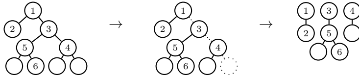
FIGURE 8. The bijection from \mathcal{T}_n^* to \mathcal{F}_n .
