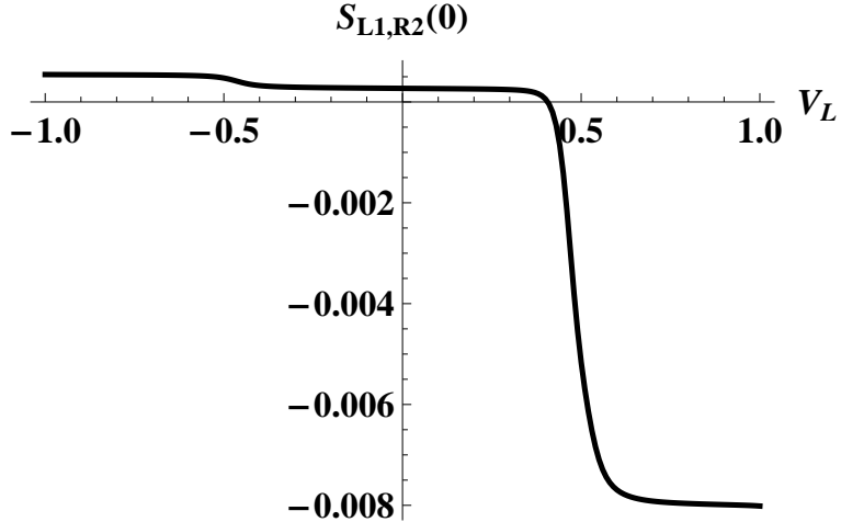
FIG. 12: Current-current crossed correlation S_{L1,R2}(0) (between I_{L1} and I_{R2} ) at zero frequency (arbitrary unit) as a function of the voltage of the left lead V_L for the same setup as in Fig. 10.
