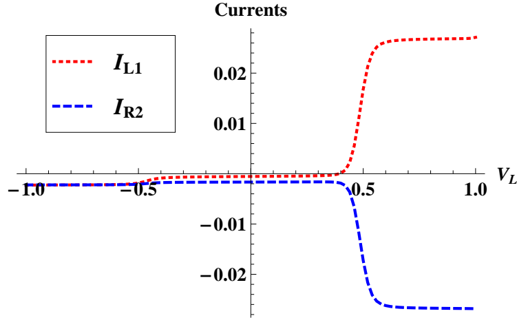
FIG. 10: (Color online) Currents (arbitrary unit) as a function of the voltage of the left normal lead V_L for \epsilon_1 = 0.5 , \epsilon_2 = 0.5 , V_R = -0.7 , \beta = 100 , t_{L1} = t_{R2} = t_{S1} = t_{S2} = 0.2 and t_{L2} = t_{R1} = 0 .
