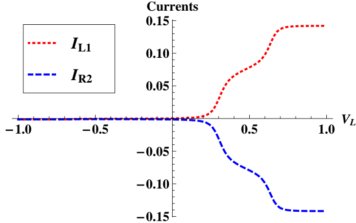
FIG. 17: (color online) Currents (arbitrary unit) as a function of the voltage of the left normal lead V_L for \epsilon_1 = 0.5 , \epsilon_2 = 0.5 , V_R = -0.7 , \beta = 100 , t_{L1} = t_{R2} = t_{S1} = t_{S2} = 0.2 , t_{L2} = t_{R1} = 0 and the tunneling between the dots t_d = 0.2 .
