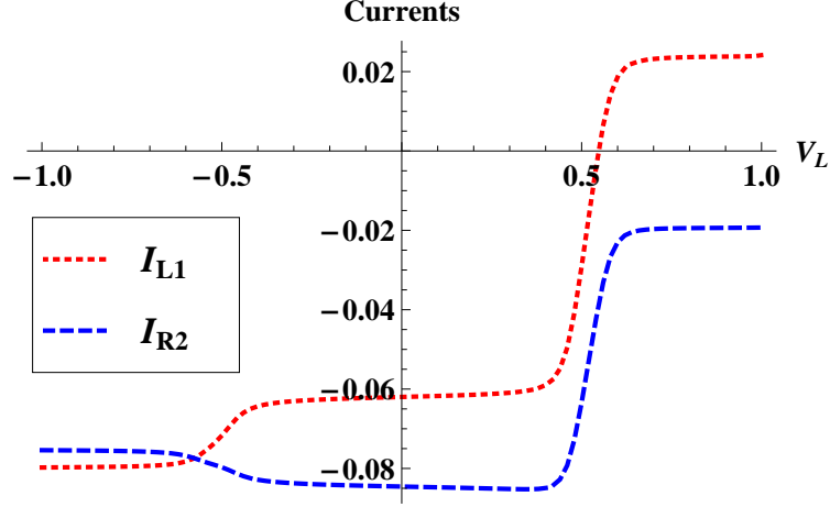
FIG. 14: (color online) Currents (arbitrary unit) as a function of the voltage of the left normal lead V_L for \epsilon_1 = 0.5 , \epsilon_2 = -0.5 , V_R = -0.7 , \beta = 100 , t_{L1} = t_{R2} = t_{S1} = t_{S2} = 0.2 , t_{L2} = t_{R1} = 0 and the tunneling between the dots t_d = 0.2 .
