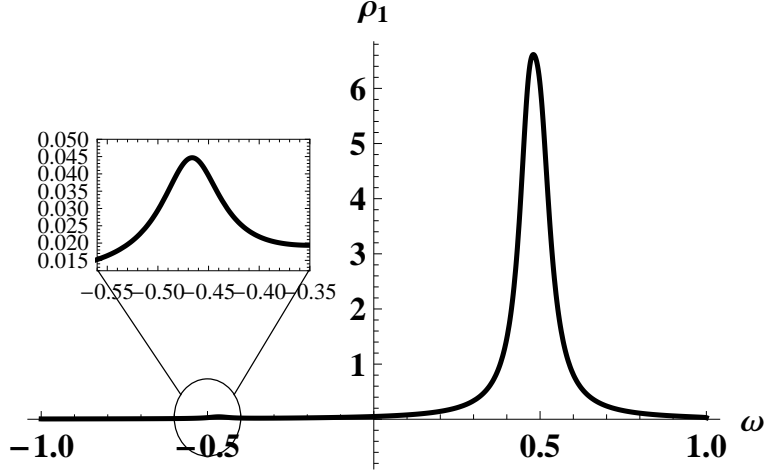
FIG. 11: Density of states of the dot 1 (arbitrary unit) for the same setup as in Fig. 10.
