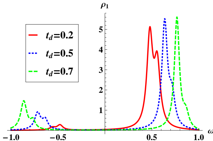
FIG. 13: (color online) Density of states of the dot 1 (arbitrary unit) for various values of the tunneling between the two dots and for \epsilon_1 = 0.5 , \epsilon_2 = -0.5 , t_{L1} = t_{R2} = t_{S1} = t_{S2} = 0.2 and t_{L2} = t_{R1} = 0 .
