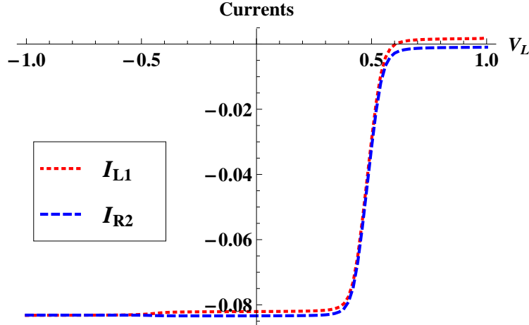
FIG. 6: (Color online) Currents (arbitrary unit) as a function of the voltage of the left normal lead V_L for \epsilon_1 = 0.5 , \epsilon_2 = -0.5 , V_R = -0.7 , \beta = 100 , t_{L1} = t_{R2} = t_{S1} = t_{S2} = 0.2 and t_{L2} = t_{R1} = 0 .
