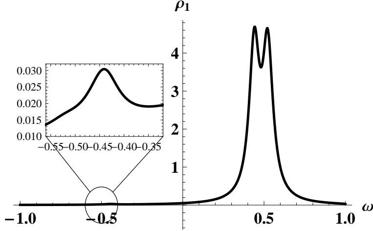
FIG. 7: Density of states of the dot 1 (arbitrary unit) for the same setup as in Fig. 6.
