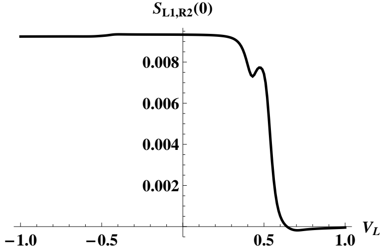
FIG. 8: Current-current crossed correlation S_{L1,R2}(0) (between I_{L1} and I_{R2} ) at zero frequency (arbitrary unit) as a function of the voltage of the left lead V_L for the same setup as in Fig. 6.
