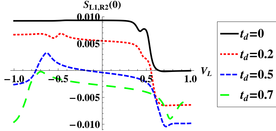
FIG. 15: (color online) Current-current crossed correlation S_{L1,R2}(0) (between I_{L1} and I_{R2} ) at zero frequency (arbitrary unit) as a function of the voltage of the left lead V_L for various values of the tunneling between the two dots and for \epsilon_1 = 0.5 , \epsilon_2 = -0.5 , V_R = -0.7 , \beta = 100 , t_{L1} = t_{R2} = t_{S1} = t_{S2} = 0.2 and t_{L2} = t_{R1} = 0 .
