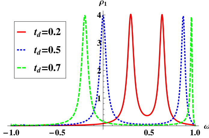
FIG. 16: (color online) Density of states of the dot 1 (arbitrary unit) for various values of the tunneling between the two dots and for \epsilon_1 = 0.5 , \epsilon_2 = 0.5 , t_{L1} = t_{R2} = t_{S1} = t_{S2} = 0.2 and t_{L2} = t_{R1} = 0 .
