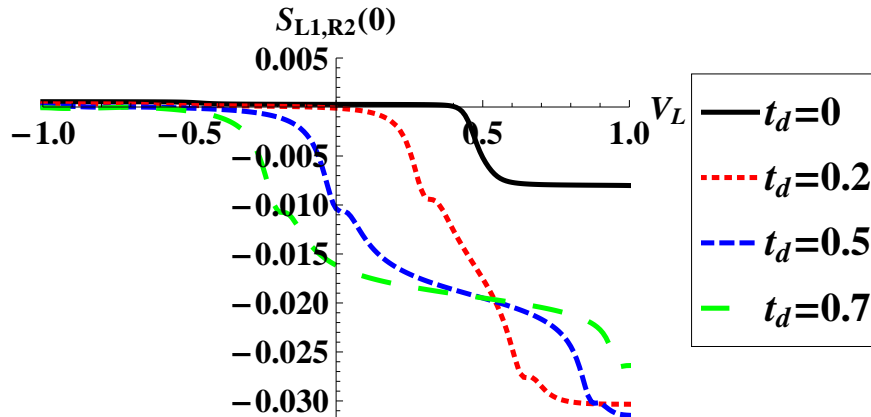
FIG. 18: (color online) Current-current crossed correlation S_{L1,R2}(0) (between I_{L1} and I_{R2} ) at zero frequency (arbitrary unit) as a function of the voltage of the left lead V_L for various values of the tunneling between the two dots and for \epsilon_1 = 0.5 , \epsilon_2 = 0.5 , V_R = -0.7 , \beta = 100 , t_{L1} = t_{R2} = t_{S1} = t_{S2} = 0.2 and t_{L2} = t_{R1} = 0 .
