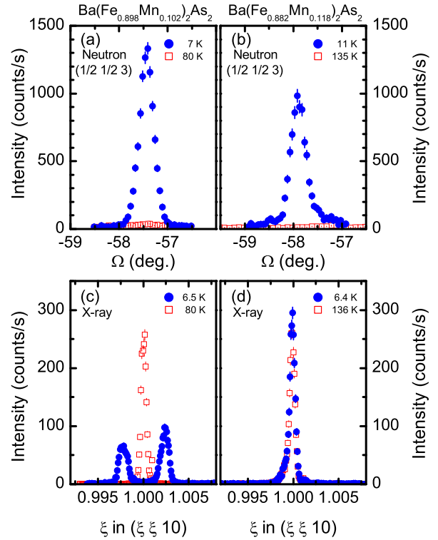
FIG. 2: Neutron diffraction rocking scans through the (\frac{1}{2} \frac{1}{2} 3) magnetic Bragg peak above (open squares) and below (filled circles) the AFM transition for (a) \text{Ba}(\text{Fe}_{0.898}\text{Mn}_{0.102})_2\text{As}_2 and (b) \text{Ba}(\text{Fe}_{0.882}\text{Mn}_{0.118})_2\text{As}_2 . Panels (c) and (d) show scans along the (\xi, \xi, 0) direction through the (1 1 10) charge reflection above (open squares) and below (filled circles) the AFM transition for these samples. Note the splitting for the x = 0.102 sample and its absence for x = 0.118 .
