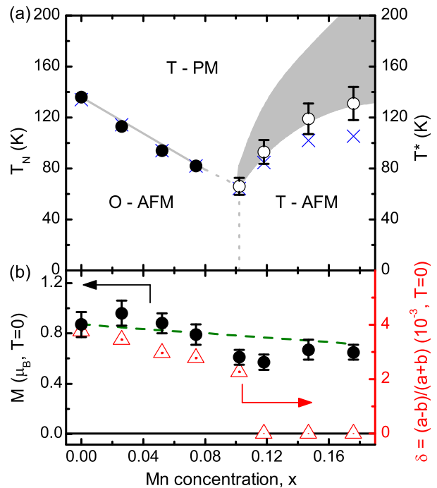
FIG. 4: (Color online) (a) The compositional phase diagram for \text{Ba}(\text{Fe}_{1-x}\text{Mn}_x)_2\text{As}_2 determined from neutron and x-ray diffraction measurements. Closed circles denote T_N and open circles represent T^* as described in the text. Crosses denote the temperature corresponding to minima of \frac{dR}{dT} found in Fig. 1. The shaded region denotes the extent of the magnetic scattering above T^* . The vertical dashed line marks the approximate composition for the change from an orthorhombic to tetragonal structure. (b) The measured magnetic moment and structural distortion as a function of Mn-doping. The dashed line represents the value of the magnetic moment per Fe atom rather than Fe/Mn site as a function of Mn-doping.
