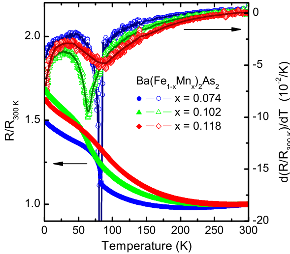
FIG. 1: (Color online) Resistance, normalized to the value at T = 300 K, and the temperature derivative of the resistance ratio for the x = 0.074 , 0.102 and 0.118 samples. Lines are guides to the eye.
