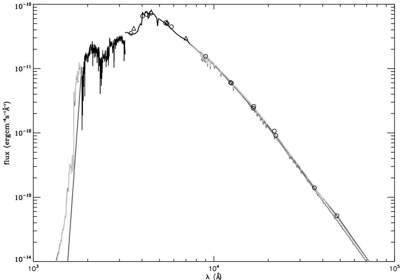
Fig. 2. The whole spectrum obtained for \gamma Equ. Black line corresponds to the average of the IUE spectra and to the Kharitonov et al. 1988's spectrum. For wavelengths \lambda < 1854 \text{ \AA} and \lambda > 7390 \text{ \AA} , the figure shows the curve obtained using the interpolation method (dark grey line), the Kurucz model that best fits the spectroscopy in the visible and the photometry in the infrared when models are calibrated with the star's magnitude m_V (grey line) and when models are calibrated with the relation (R/d)^2 (light grey line). The Geneva and infrared photometry from Table 4 (circles) and Johnson UBVRI photometry (triangles) are overplotted to the spectrum.
