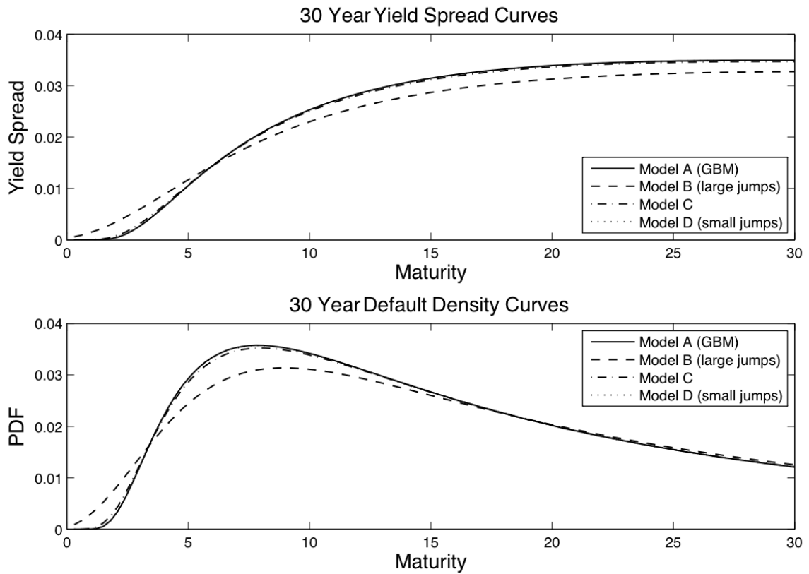
Figure 1: Thirty year yield spread and default PDF curves for geometric Brownian motion model and three versions of the VG TCBM credit risk model.
