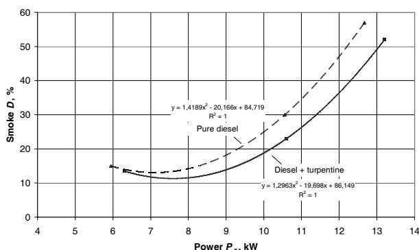
Fig 5. Dependence of exhaust gas smoke on the engine power for run with different fuels
