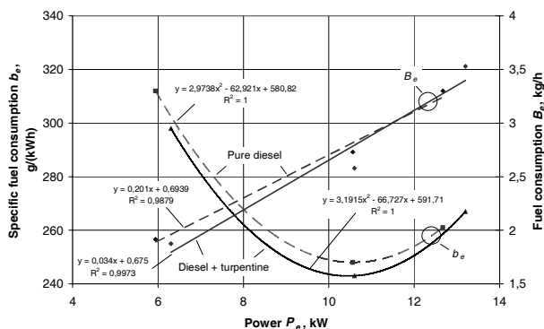
Fig 4. Dependence of fuel consumption on the engine power for run at speed of 1 200 min -1
