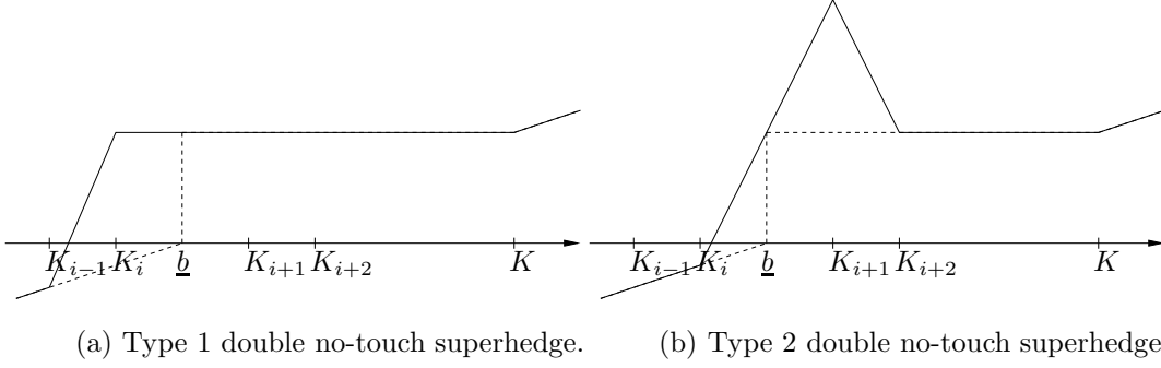
Figure 5: Two possible superhedges \overline{H}_1^{II}(K), \overline{H}_2^{II}(K) of the double no-touch when calls and digitals at the barrier are not traded.
