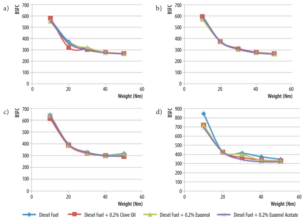
Fig. 17. BSFC of diesel fuel, diesel fuel+0.2% clove oil, diesel fuel+0.2% eugenol and diesel fuel+0.2% eugenyl acetate at: a – 1500 rpm; b – 2000 rpm; c – 2500 rpm; d – 3000 rpm
