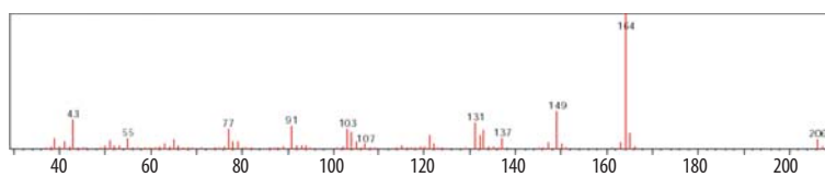
Fig. 14. MS spectra of the second peak
