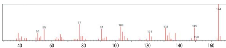
Fig. 13. MS spectra of the first peak
