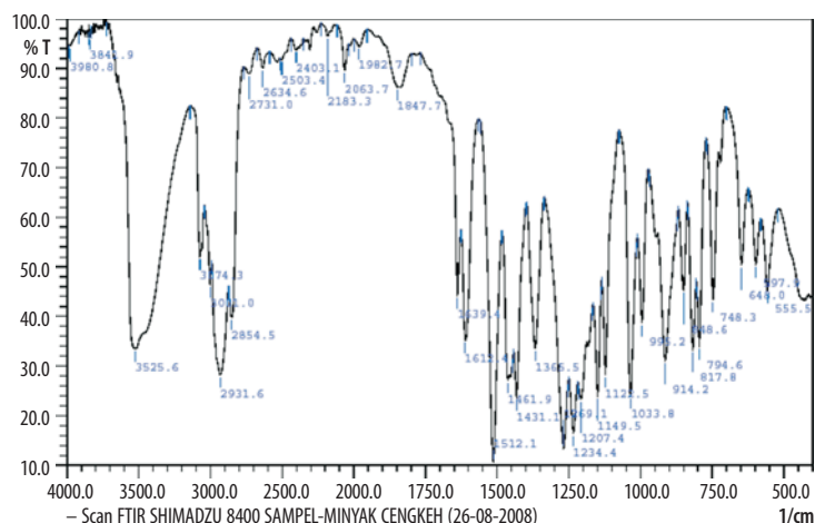
Fig. 5. IR spectra of clove oil
