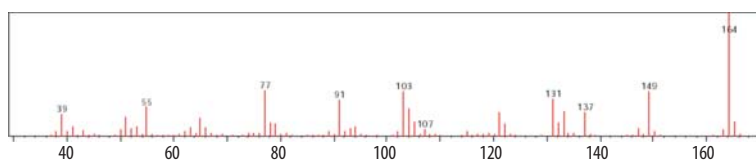
Fig. 6. MS spectra of the second peak
