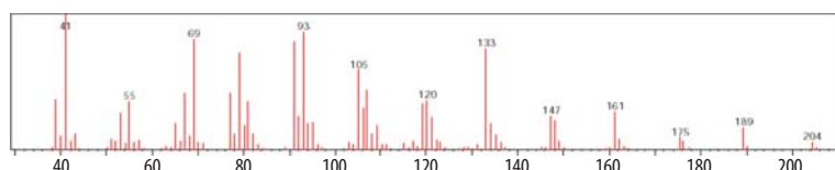
Fig. 7. MS spectra of the third peak
