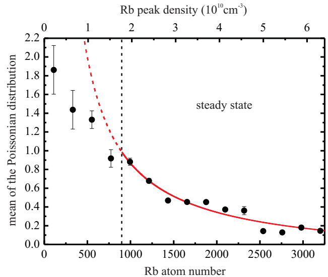
FIG. 4: (Color online) Mean of the Poissonian distribution of Cs atom numbers as a function of the Rb atom number and peak density. The red solid line is a fit of equation (2) to the data within the steady state regime. The red dashed line is the extrapolation to the non-steady state regime of the Cs MOT.
