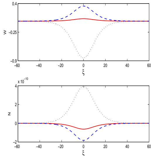
FIG. 3: (Color online) Whistler solitary solution of Eqs. (28) and (29) with associated electric field W (upper panel) and density perturbation N (lower panel) for \omega = 0.4 (solid line) and 0.38 (dashed and dotted line). The other parameter values are B_0 = 5 \times 10^8 \text{T} , n_0 = 10^{36} \text{m}^{-3} (for solid and dashed line) and 2.1 \times 10^{36} \text{m}^{-3} (for dotted line), \Theta = 0.2 . The values of M are M = 35.38 (for solid and dashed line) and 22.23 (for dotted line).
