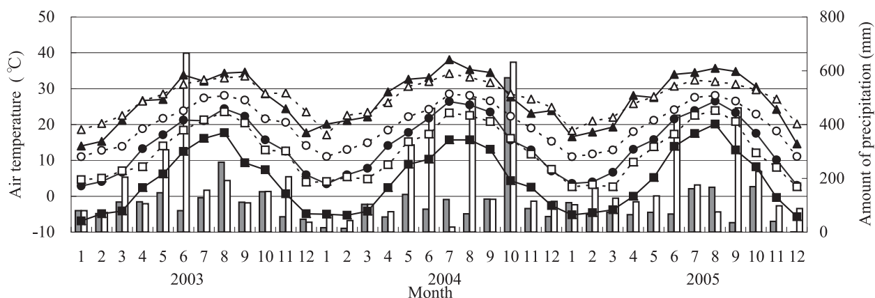
Fig. 1. Meteorological data for Tsukuba and Tanegashima
