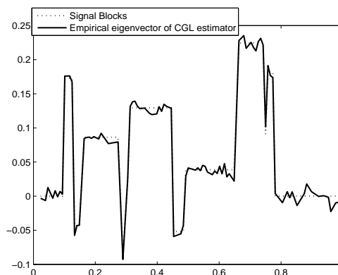
Figure 9(b). Signal Blocks and Eigenvector associated to the largest eigenvalue of \hat{\Sigma}_{\hat{\lambda}}
