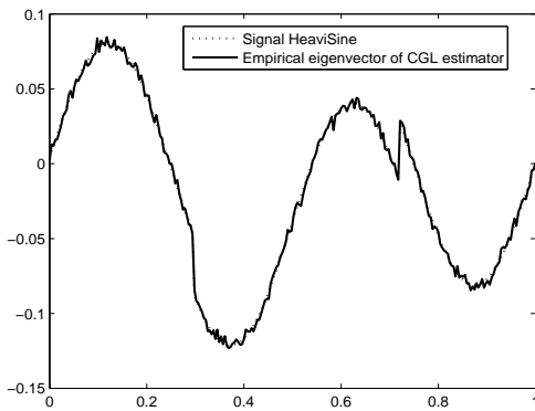
Figure 2(a). Signal HeaviSine and Eigenvector associated to the largest eigenvalue of \widehat{\Sigma}_{\lambda}
