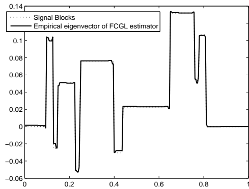
Figure 3(b). Signal Blocks and Eigenvector associated to the largest eigenvalue of \widehat{\Sigma}_{\hat{\lambda}}
