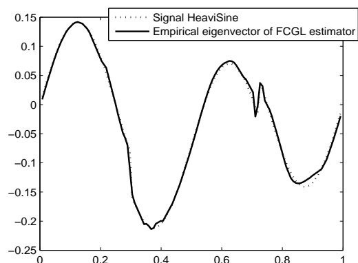
Figure 10(a). Signal HeaviSine and Eigenvector associated to the largest eigenvalue of \hat{\Sigma}_{\hat{f}}
