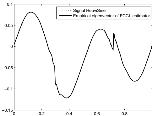
Figure 3(a). Signal HeaviSine and Eigenvector associated to the largest eigenvalue of \widehat{\Sigma}_{\hat{\lambda}}
