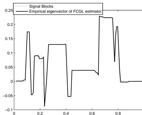
Figure 10(b). Signal Blocks and Eigenvector associated to the largest eigenvalue of \hat{\Sigma}_{\hat{f}}
