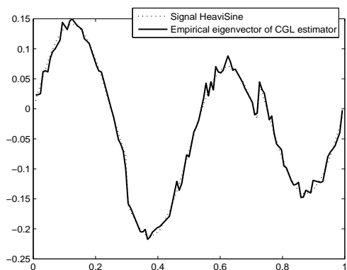
Figure 9(a). Signal HeaviSine and Eigenvector associated to the largest eigenvalue of \hat{\Sigma}_{\hat{\lambda}}
