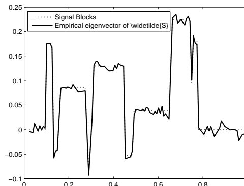
Figure 8(b). Signal Blocks and Eigenvector associated to the largest eigenvalue of \tilde{S}
