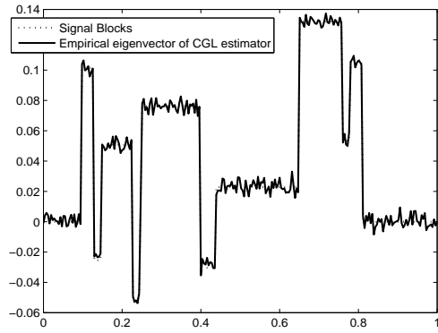
Figure 2(b). Signal Blocks and Eigenvector associated to the largest eigenvalue of \widehat{\Sigma}_{\lambda}
