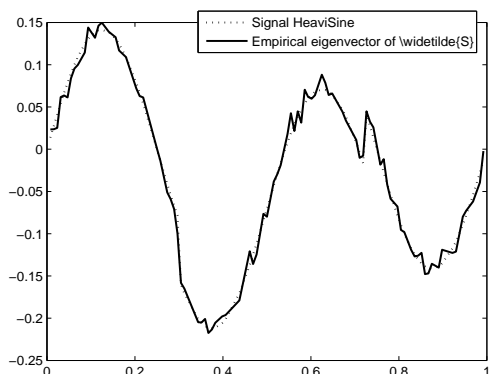
Figure 8(a). Signal HeaviSine and Eigenvector associated to the largest eigenvalue of \tilde{S}
