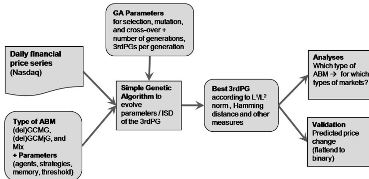
Figure 1: demonstrates a process overview of how a time series of daily adjusted closing prices is fed to a GA along with different parameters determining (i) the type of ABM for the 3PG which is used for generating a similar time series to the real one (during the in-sample period) and (ii) the convergence behavior of the GA for the search of the best - most similar - 3PG according to measurements like L^1 , L^2 and the Hamming distance. This result is then analyzed with respect to the types of ABMs present in which types of markets. The generating process is validated by the accuracy of one-step predictions.
