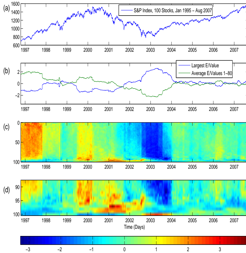
Fig. 2. (a) S&P Index (b) Normalised Largest Eigenvalue vs. Average of 80 smallest normalised eigenvalues (c) All Normalised Eigenvalues (d) Largest 12 Normalised Eigenvalues
