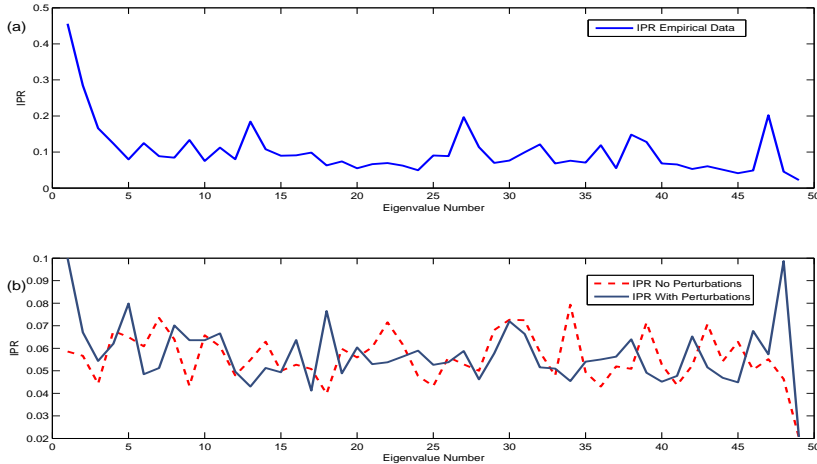
Fig. 7. (a) IPR Empirical Data (b) IPR Simulated Data
