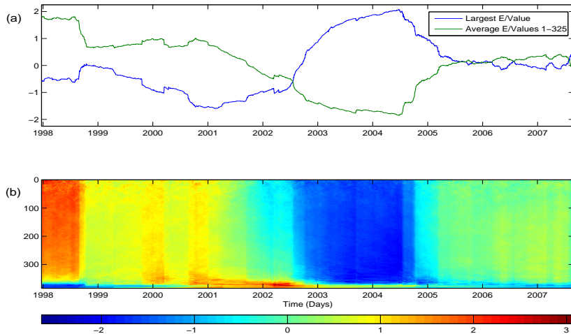
Fig. 4. (a) Normalised Largest Eigenvalue vs. Average of 325 smallest normalised eigenvalues (b) All Normalised Eigenvalues
