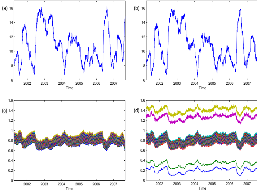
Fig. 6. (a) Largest Eigenvalue, one factor model (b) Largest Eigenvalue, Market plus sectors model (c) Eigenvalues 1-48, one factor model (d) Eigenvalues 1-48, Market plus sectors model
