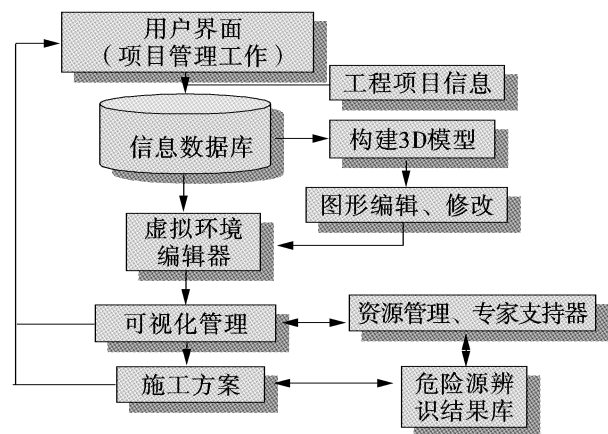
图1 虚拟现实施工方案设计示意图 Fig.1 Skeleton sketch of construction plan based on Virtual Reality
