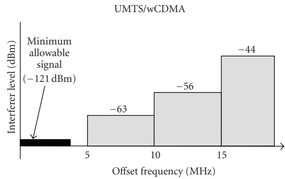
FIGURE 4: wCDMA receiver interference profile.
