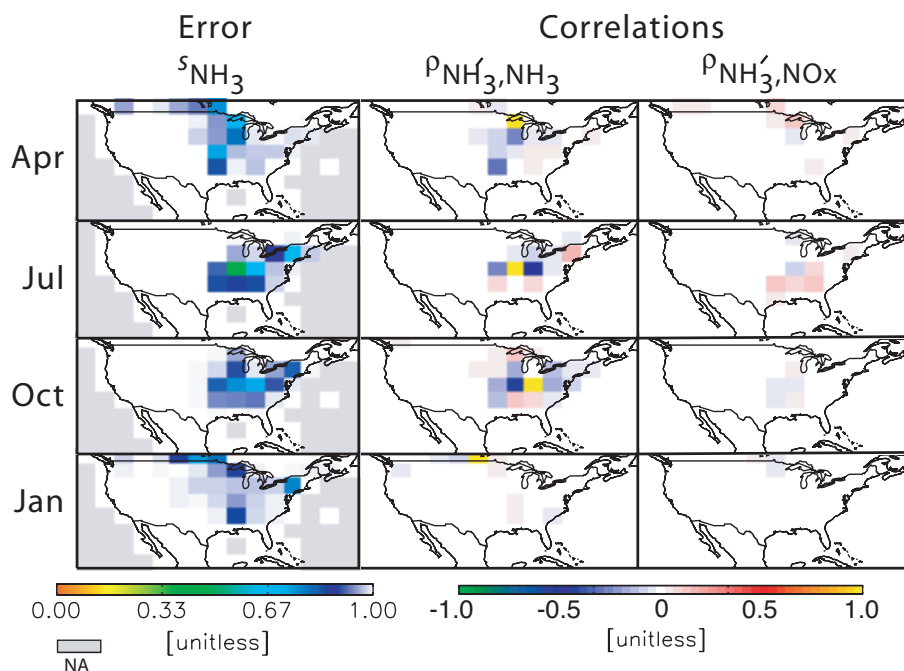
Fig. 12. The left column gives the standard error estimate of the optimized scaling factors for anthropogenic NH 3 emissions, s_{\text{NH}_3} . The center column shows the correlation of the scaling factor for anthropogenic NH 3 emissions with the least uncertainty (NH 3 ) with other scaling factors for the same inventory. The right column shows the correlation of the scaling factors for the anthropogenic NH 3 emissions with the least uncertainty (NH 3 ) with the scaling factors for surface emissions of NO x .
