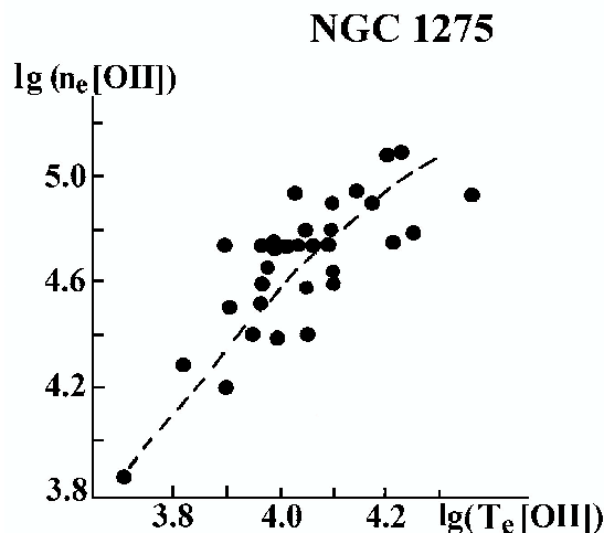
Fig. 1. \log T_e vs. \log n_e in the zone of [O II] lines in the NGC 1275 nucleus in the 1971–1976 monitoring.
